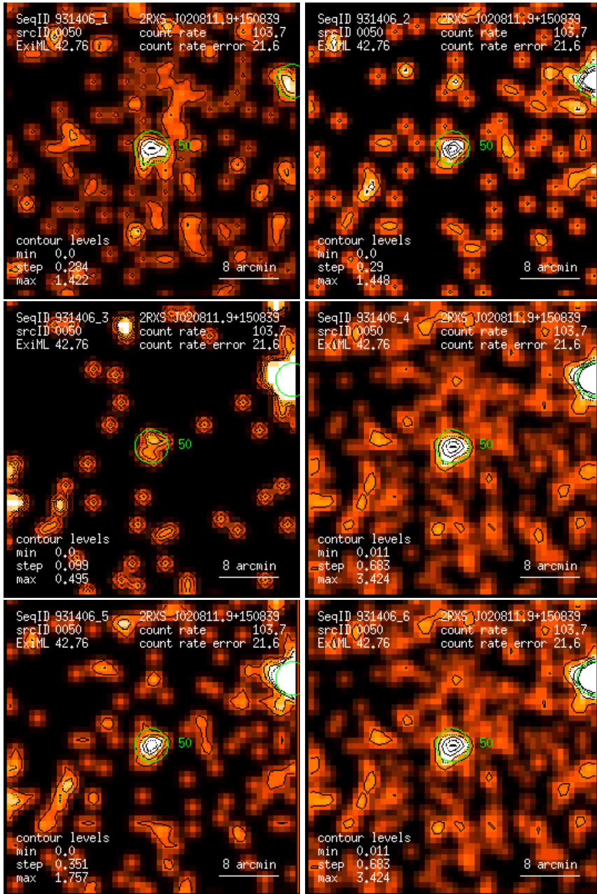
Figure 50: RASS 931406: detection 0050: band rate images, Gaussian filter: (1) PSPC channels 11 – 41, (2) 52 – 90, (3) 91 – 201, (4) 11 – 235, (5) 52 – 201, (6) 11 – 201. Broad band rates in counts/ks. Band rate contour levels in counts/ks/arcmin 2 .
