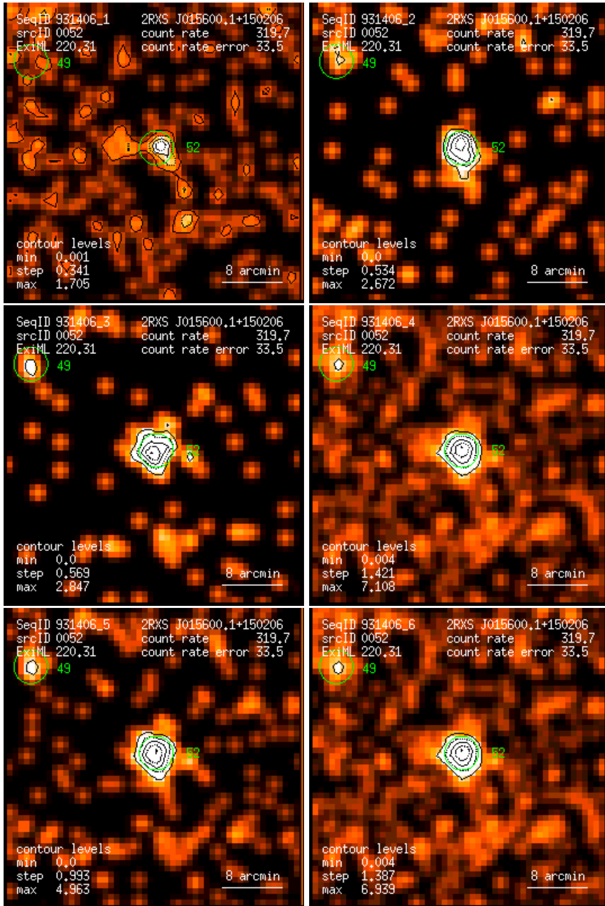
Figure 52: RASS 931406: detection 0052: band rate images, Gaussian filter: (1) PSPC channels 11 – 41, (2) 52 – 90, (3) 91 – 201, (4) 11 – 235, (5) 52 – 201, (6) 11 – 201. Broad band rates in counts/ks. Band rate contour levels in counts/ks/arcmin 2 .
