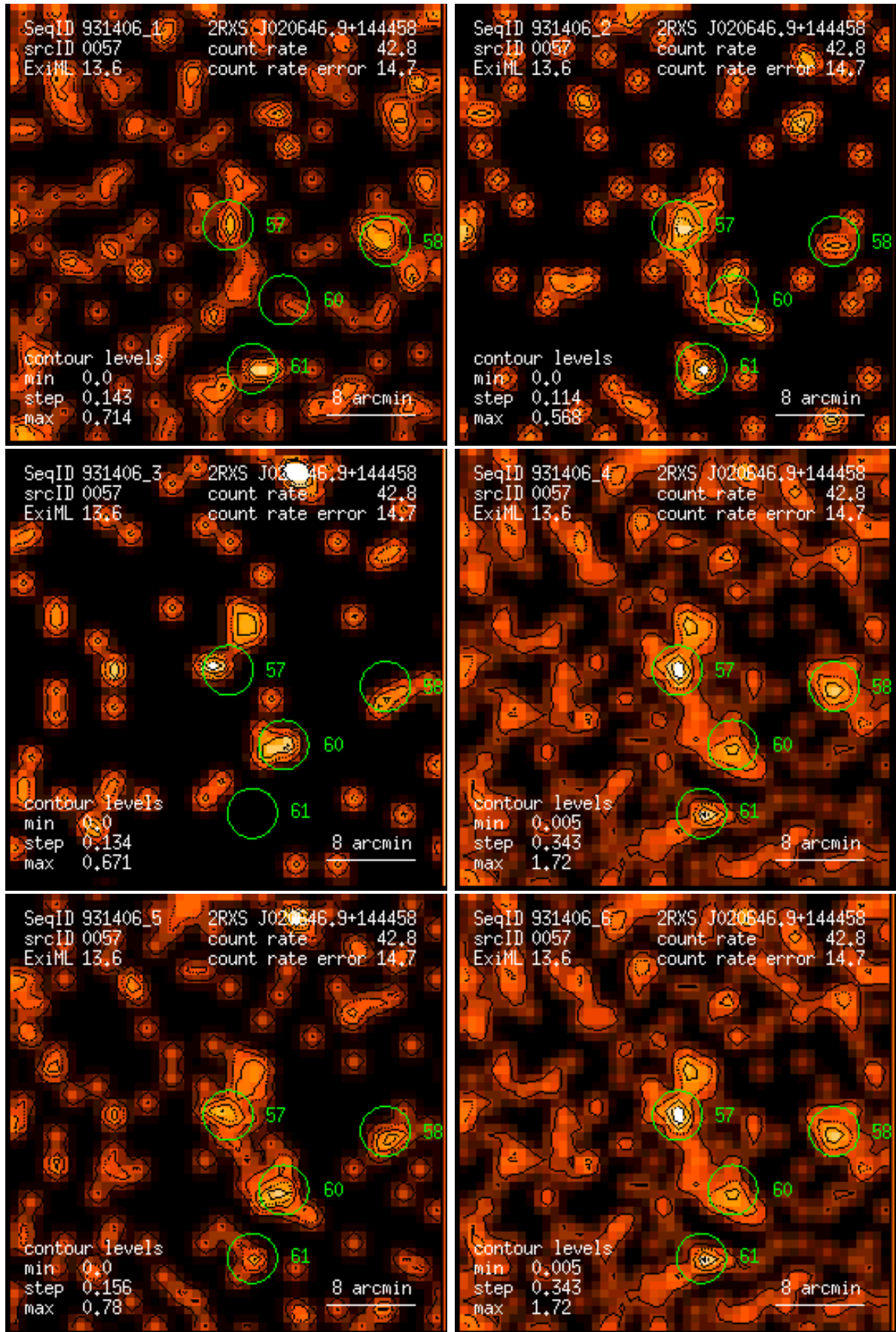
Figure 57: RASS 931406: detection 0057: band rate images, Gaussian filter: (1) PSPC channels 11 – 41, (2) 52 – 90, (3) 91 – 201, (4) 11 – 235, (5) 52 – 201, (6) 11 – 201. Broad band rates in counts/ks. Band rate contour levels in counts/ks/arcmin 2 .
