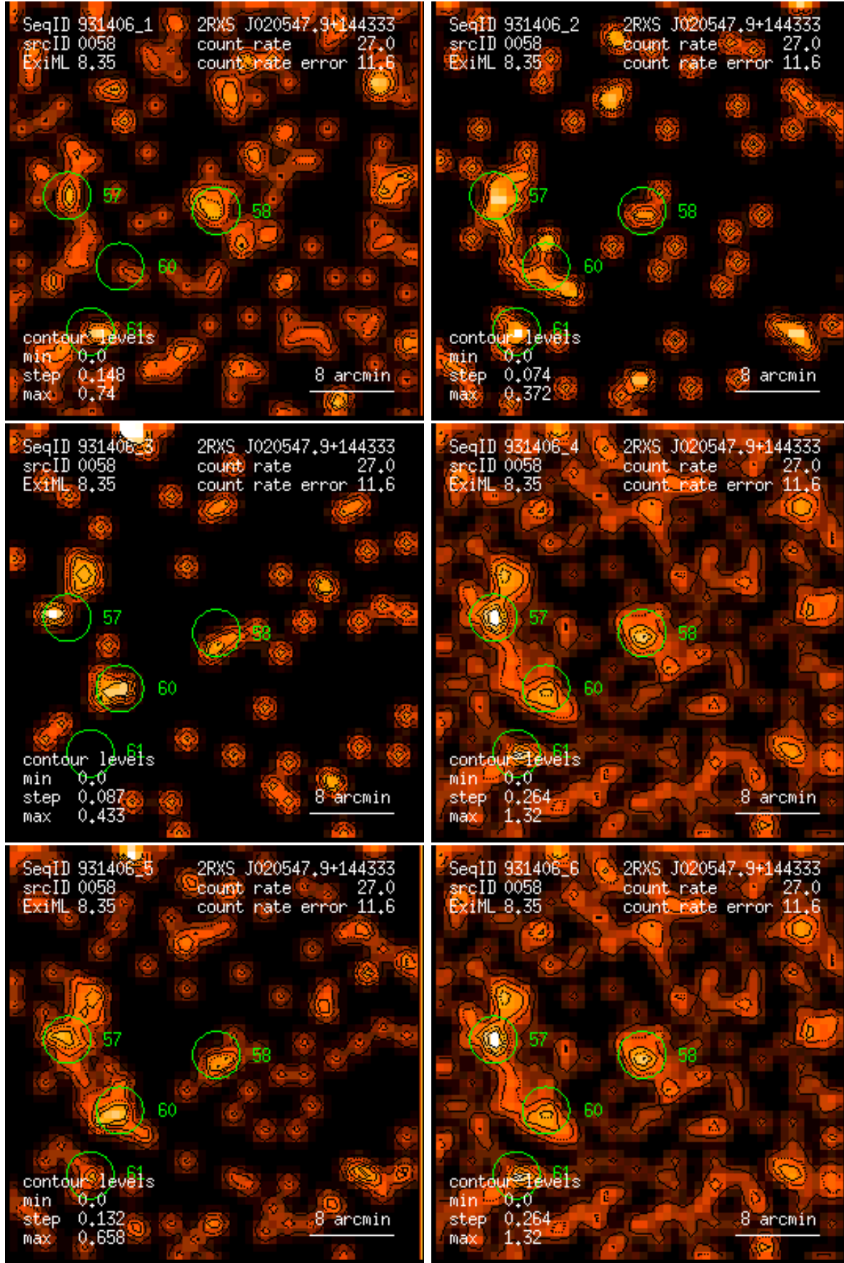
Figure 58: RASS 931406: detection 0058: band rate images, Gaussian filter: (1) PSPC channels 11 – 41, (2) 52 – 90, (3) 91 – 201, (4) 11 – 235, (5) 52 – 201, (6) 11 – 201. Broad band rates in counts/ks. Band rate contour levels in counts/ks/arcmin 2 .
