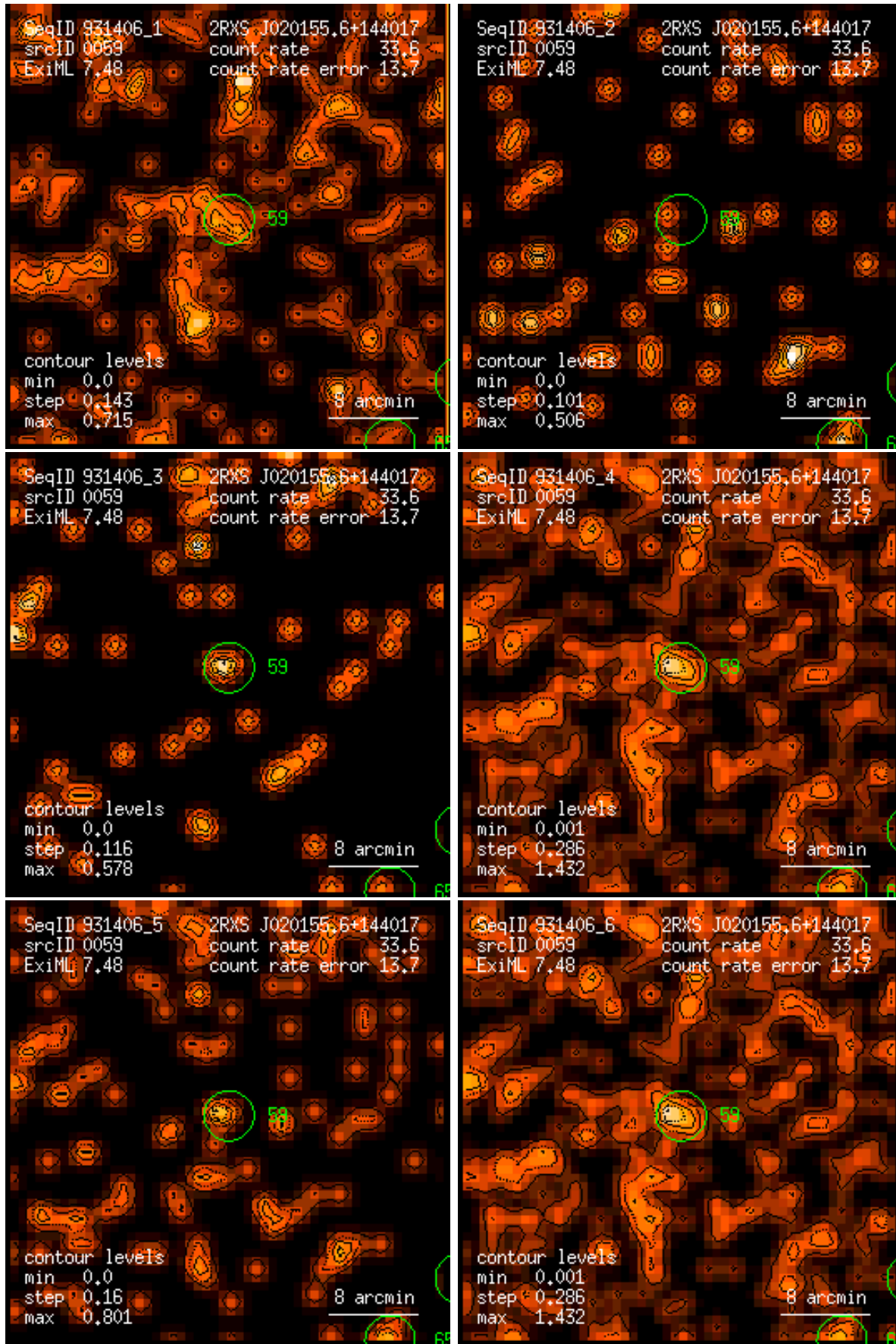
Figure 59: RASS 931406: detection 0059: band rate images, Gaussian filter: (1) PSPC channels 11 – 41, (2) 52 – 90, (3) 91 – 201, (4) 11 – 235, (5) 52 – 201, (6) 11 – 201. Broad band rates in counts/ks. Band rate contour levels in counts/ks/arcmin 2 .
