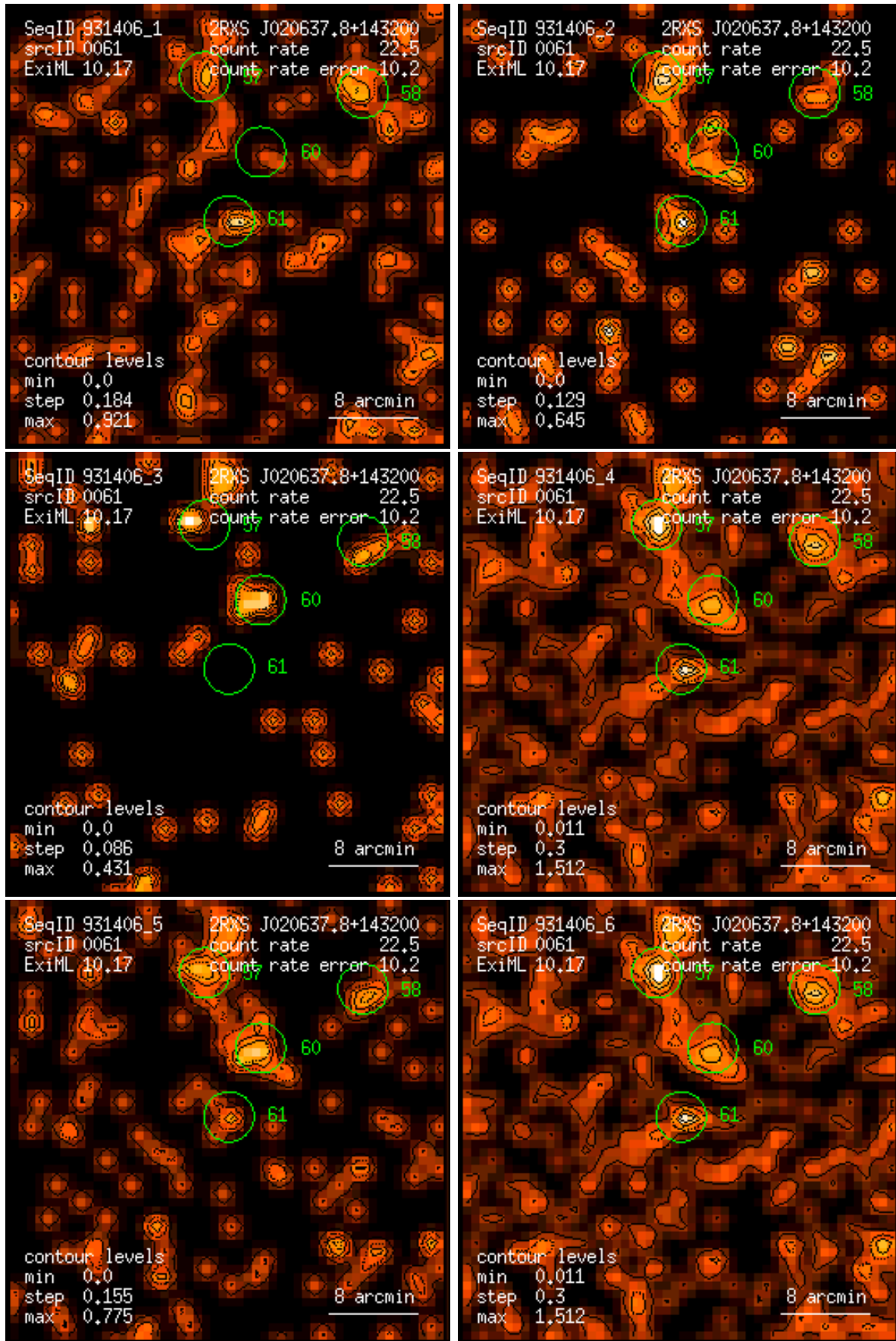
Figure 61: RASS 931406: detection 0061: band rate images, Gaussian filter: (1) PSPC channels 11 – 41, (2) 52 – 90, (3) 91 – 201, (4) 11 – 235, (5) 52 – 201, (6) 11 – 201. Broad band rates in counts/ks. Band rate contour levels in counts/ks/arcmin 2 .
