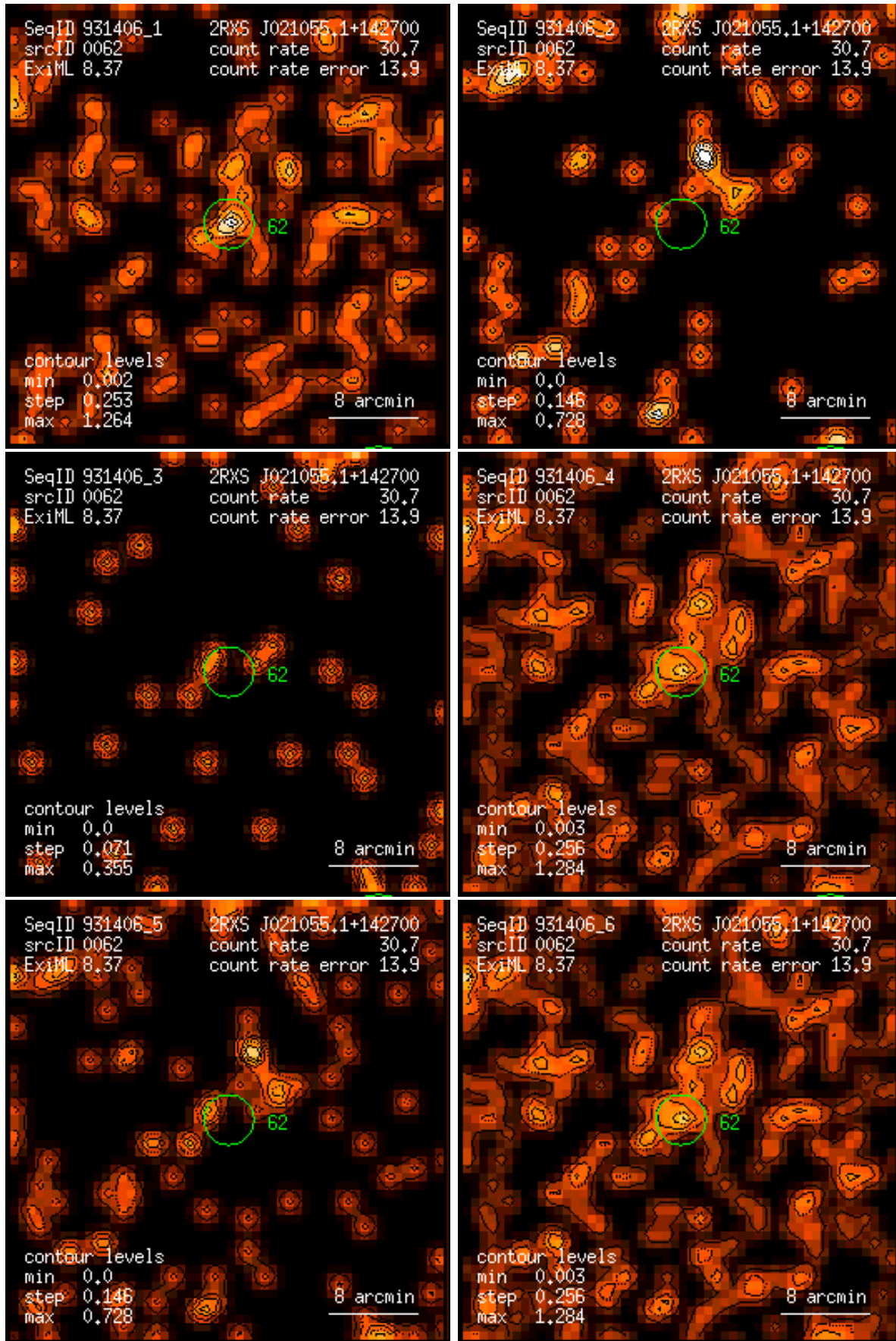
Figure 62: RASS 931406: detection 0062: band rate images, Gaussian filter: (1) PSPC channels 11 – 41, (2) 52 – 90, (3) 91 – 201, (4) 11 – 235, (5) 52 – 201, (6) 11 – 201. Broad band rates in counts/ks. Band rate contour levels in counts/ks/arcmin 2 .
