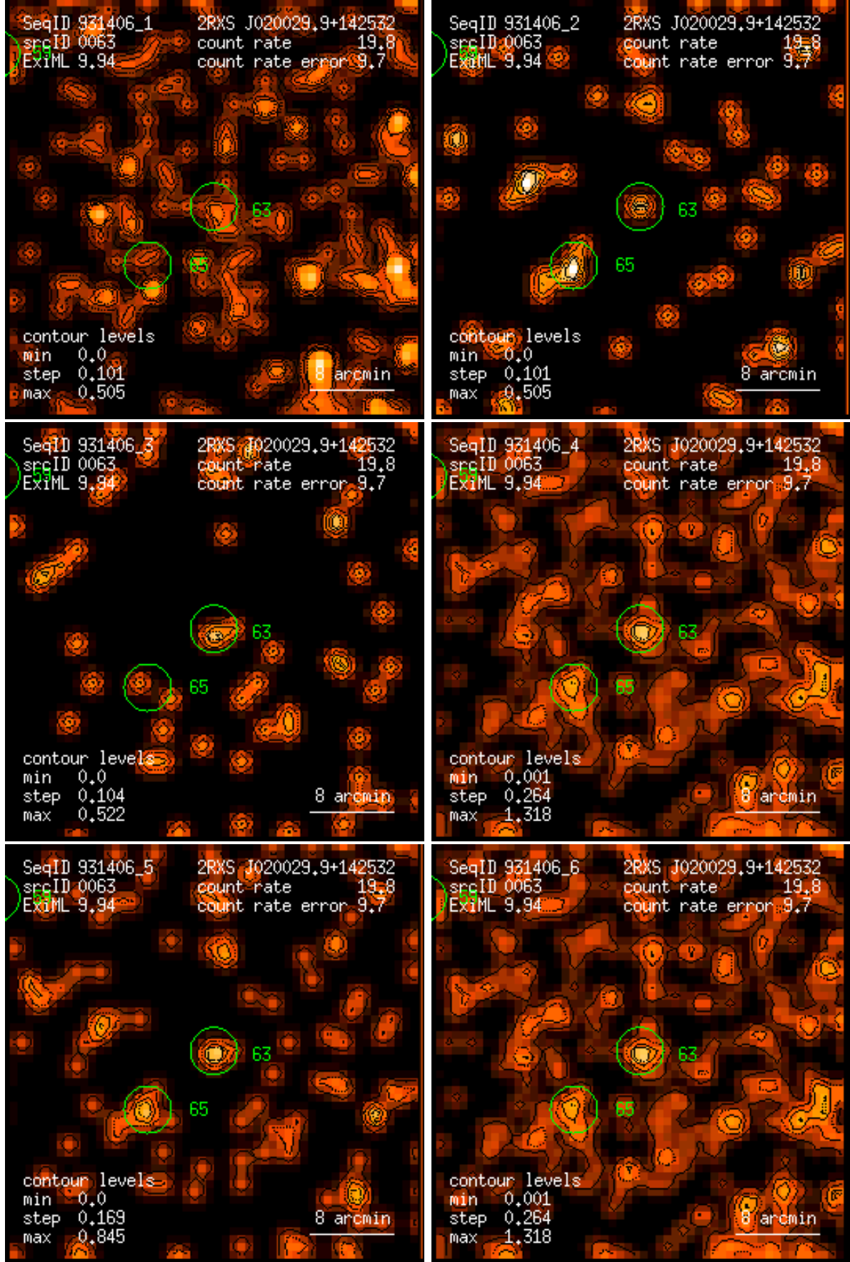
Figure 63: RASS 931406: detection 0063: band rate images, Gaussian filter: (1) PSPC channels 11 – 41, (2) 52 – 90, (3) 91 – 201, (4) 11 – 235, (5) 52 – 201, (6) 11 – 201. Broad band rates in counts/ks. Band rate contour levels in counts/ks/arcmin 2 .
