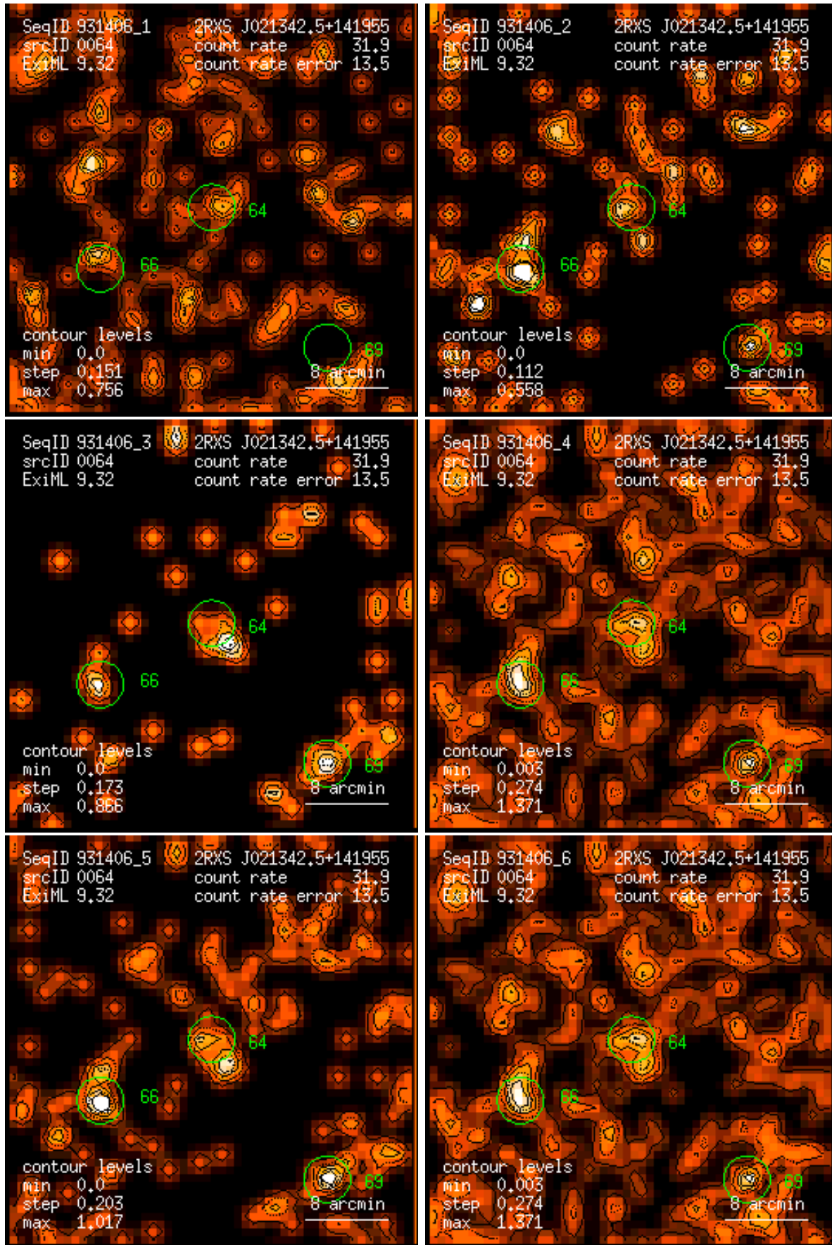
Figure 64: RASS 931406: detection 0064: band rate images, Gaussian filter: (1) PSPC channels 11 – 41, (2) 52 – 90, (3) 91 – 201, (4) 11 – 235, (5) 52 – 201, (6) 11 – 201. Broad band rates in counts/ks. Band rate contour levels in counts/ks/arcmin 2 .
