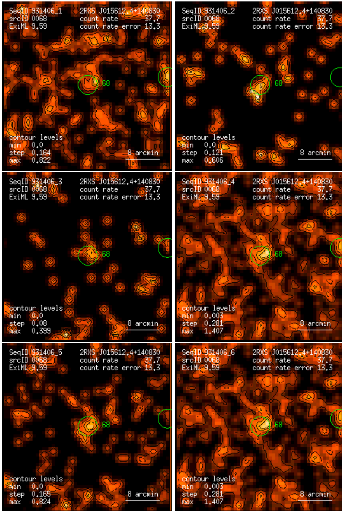
Figure 68: RASS 931406: detection 0068: band rate images, Gaussian filter: (1) PSPC channels 11 – 41, (2) 52 – 90, (3) 91 – 201, (4) 11 – 235, (5) 52 – 201, (6) 11 – 201. Broad band rates in counts/ks. Band rate contour levels in counts/ks/arcmin 2 .
