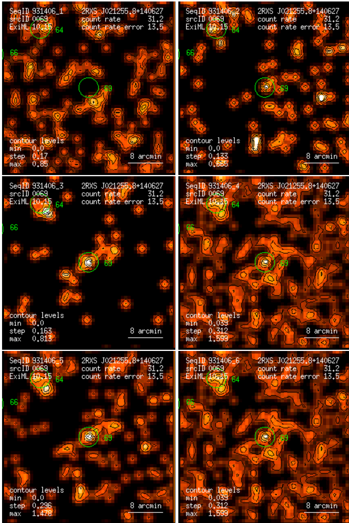
Figure 69: RASS 931406: detection 0069: band rate images, Gaussian filter: (1) PSPC channels 11 – 41, (2) 52 – 90, (3) 91 – 201, (4) 11 – 235, (5) 52 – 201, (6) 11 – 201. Broad band rates in counts/ks. Band rate contour levels in counts/ks/arcmin 2 .
