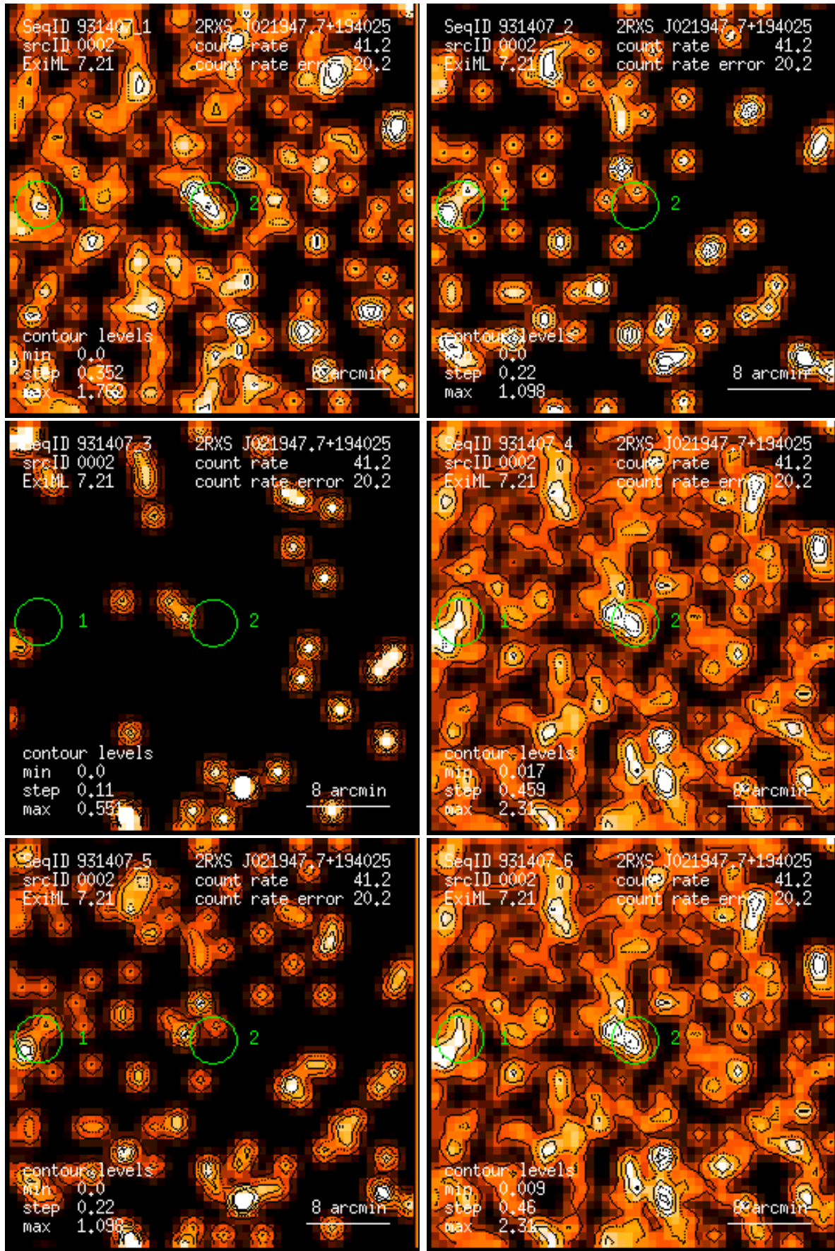
Figure 2: RASS 931407: detection 0002: band rate images, Gaussian filter: (1) PSPC channels 11 – 41, (2) 52 – 90, (3) 91 – 201, (4) 11 – 235, (5) 52 – 201, (6) 11 – 201. Broad band rates in counts/ks. Band rate contour levels in counts/ks/arcmin 2 .
