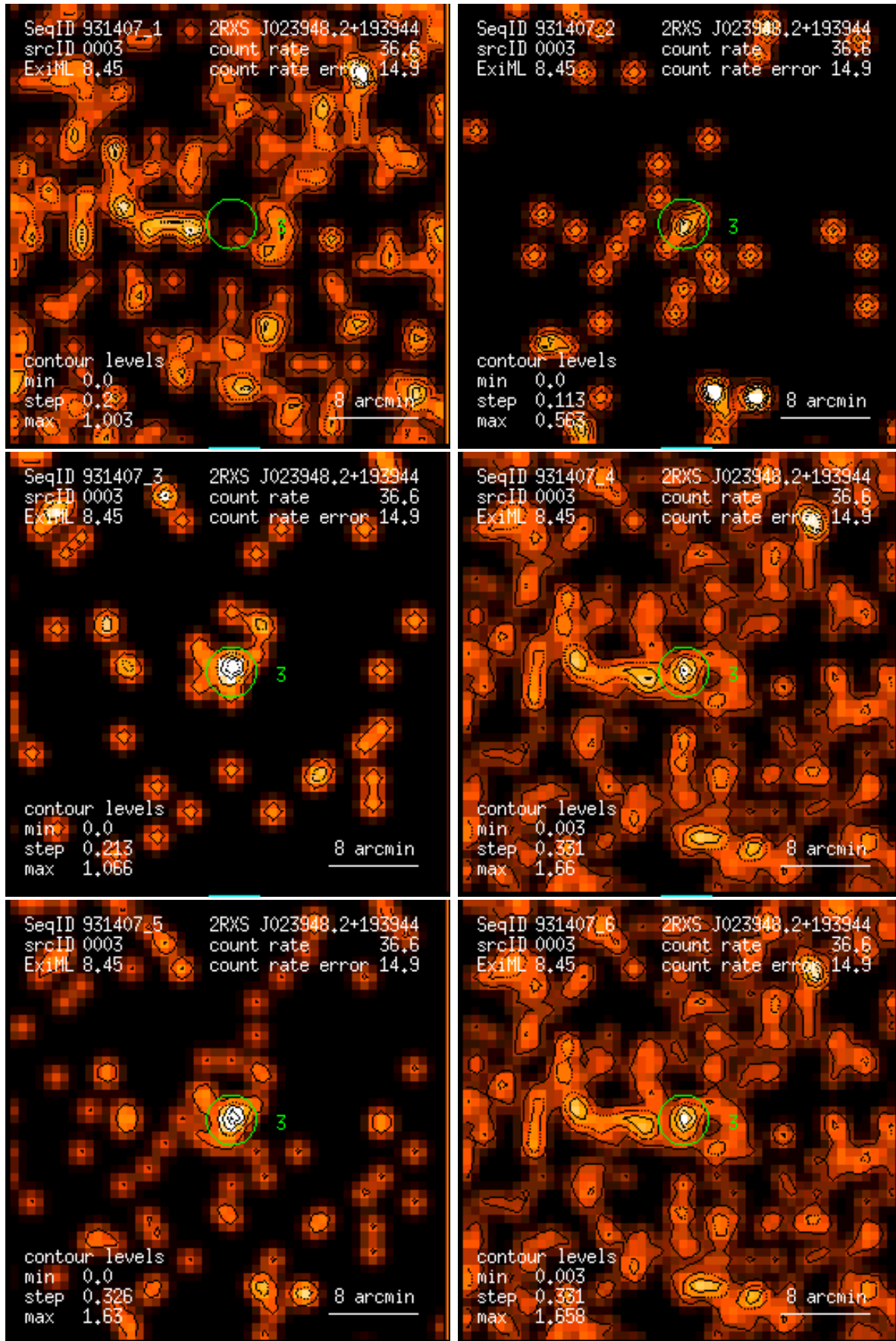
Figure 3: RASS 931407: detection 0003: band rate images, Gaussian filter: (1) PSPC channels 11 – 41, (2) 52 – 90, (3) 91 – 201, (4) 11 – 235, (5) 52 – 201, (6) 11 – 201. Broad band rates in counts/ks. Band rate contour levels in counts/ks/arcmin 2 .
