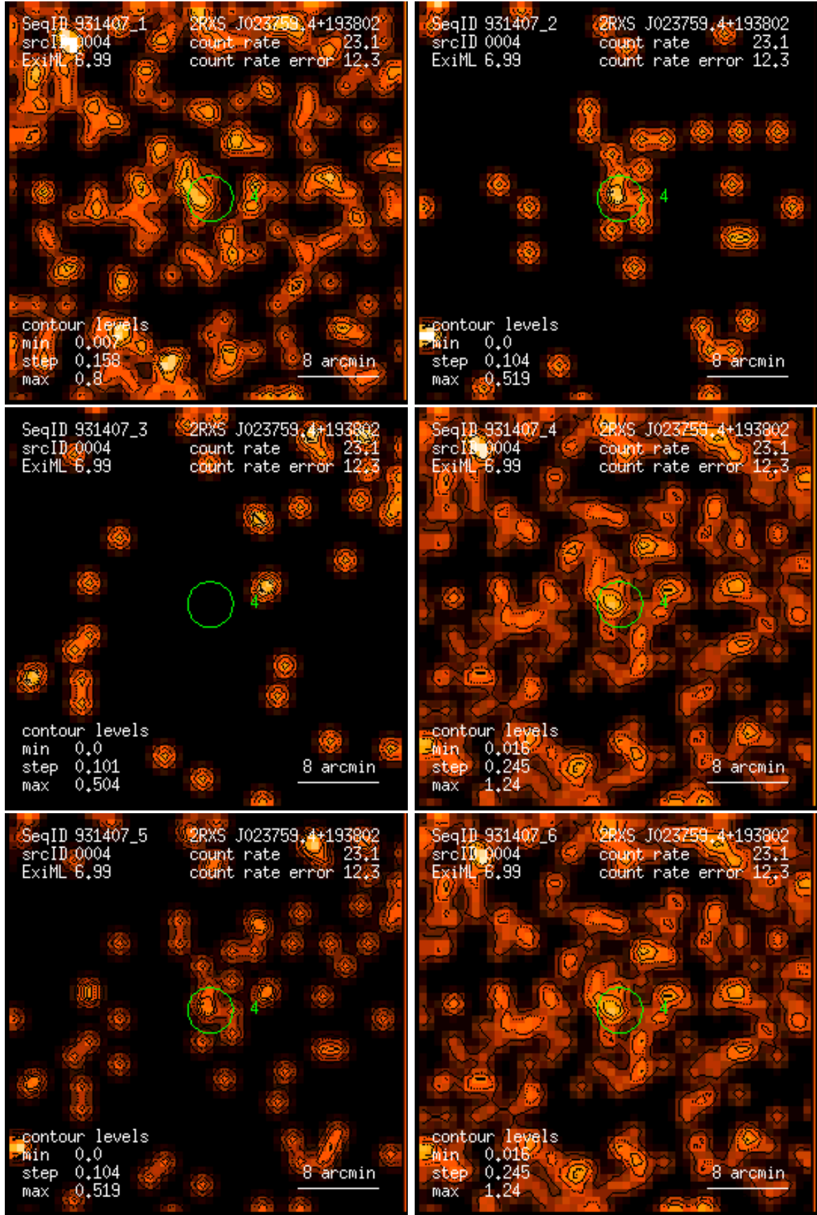
Figure 4: RASS 931407: detection 0004: band rate images, Gaussian filter: (1) PSPC channels 11 – 41, (2) 52 – 90, (3) 91 – 201, (4) 11 – 235, (5) 52 – 201, (6) 11 – 201. Broad band rates in counts/ks. Band rate contour levels in counts/ks/arcmin 2 .
