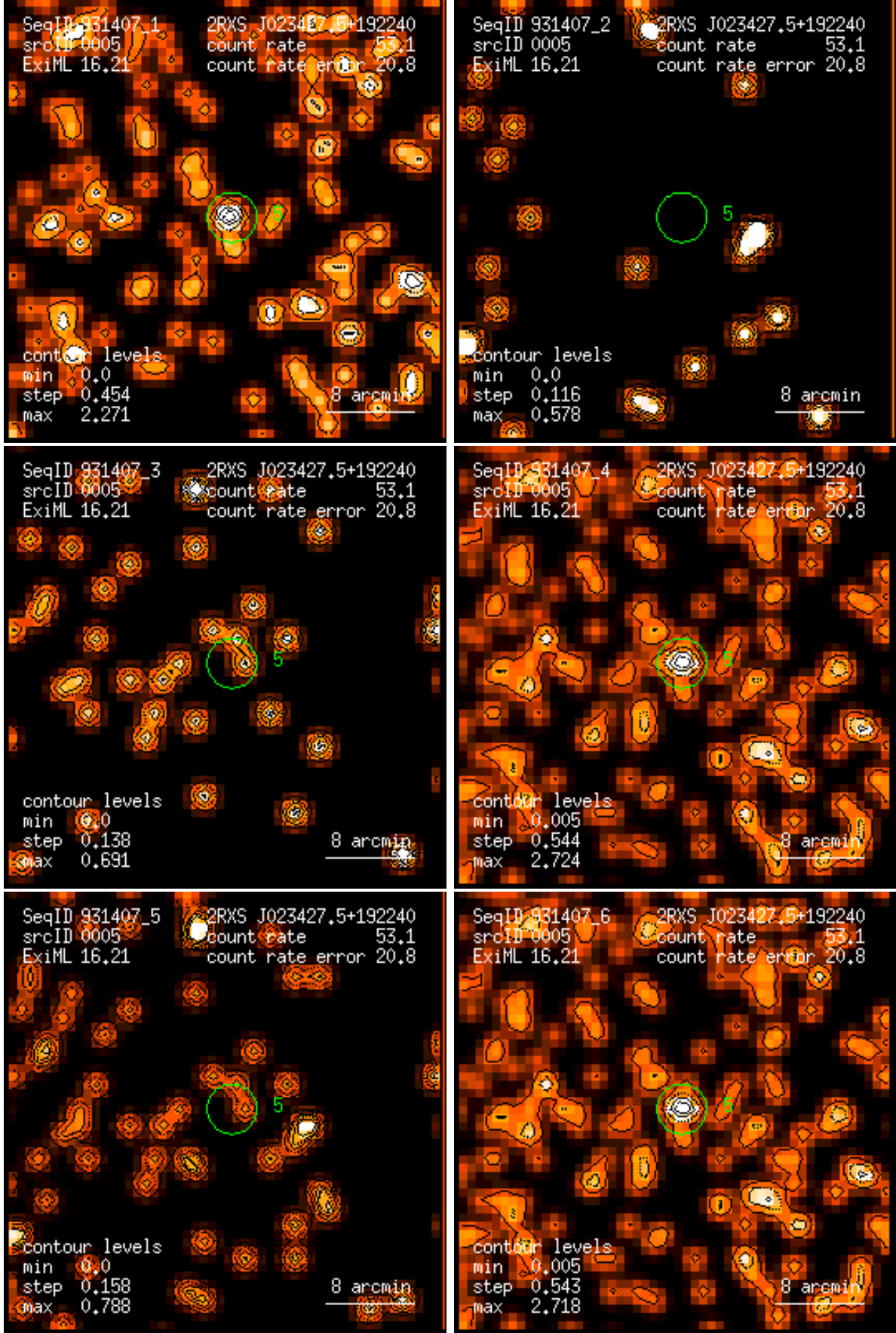
Figure 5: RASS 931407: detection 0005: band rate images, Gaussian filter: (1) PSPC channels 11 – 41, (2) 52 – 90, (3) 91 – 201, (4) 11 – 235, (5) 52 – 201, (6) 11 – 201. Broad band rates in counts/ks. Band rate contour levels in counts/ks/arcmin 2 .
