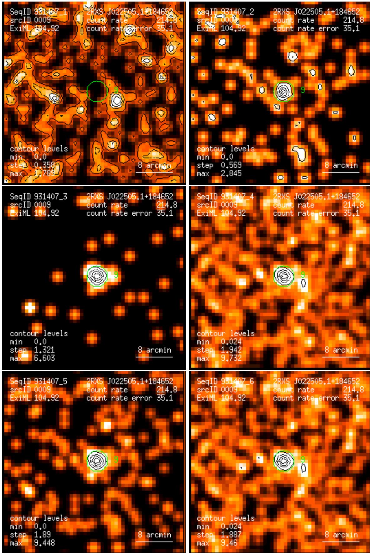
Figure 9: RASS 931407: detection 0009: band rate images, Gaussian filter: (1) PSPC channels 11 – 41, (2) 52 – 90, (3) 91 – 201, (4) 11 – 235, (5) 52 – 201, (6) 11 – 201. Broad band rates in counts/ks. Band rate contour levels in counts/ks/arcmin 2 .
