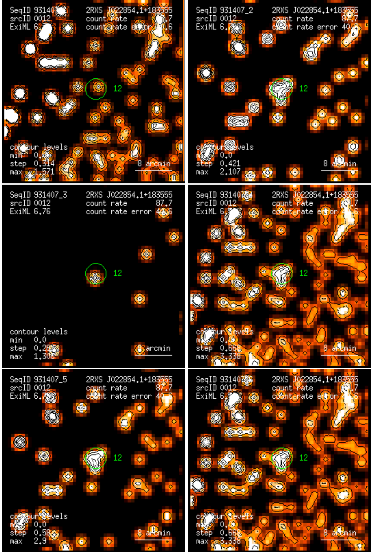
Figure 12: RASS 931407: detection 0012: band rate images, Gaussian filter: (1) PSPC channels 11 – 41, (2) 52 – 90, (3) 91 – 201, (4) 11 – 235, (5) 52 – 201, (6) 11 – 201. Broad band rates in counts/ks. Band rate contour levels in counts/ks/arcmin 2 .
