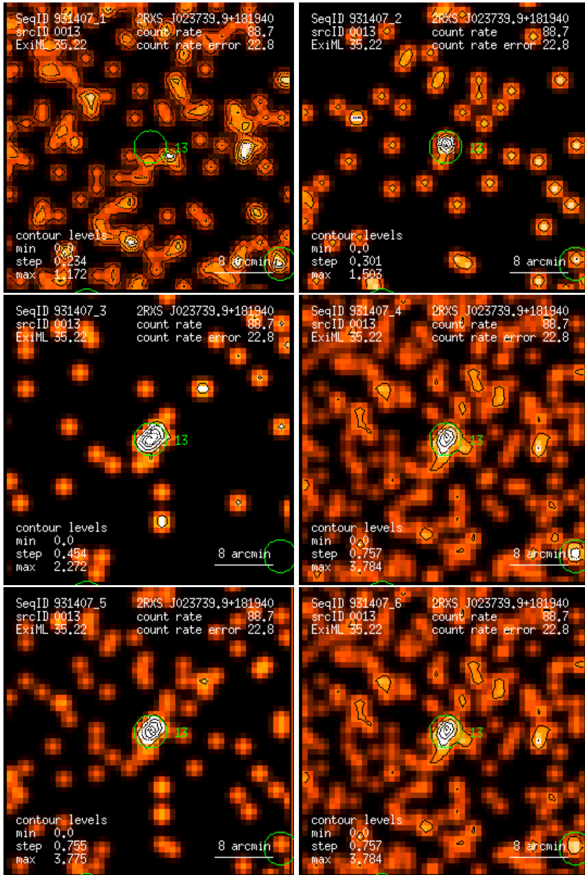
Figure 13: RASS 931407: detection 0013: band rate images, Gaussian filter: (1) PSPC channels 11 – 41, (2) 52 – 90, (3) 91 – 201, (4) 11 – 235, (5) 52 – 201, (6) 11 – 201. Broad band rates in counts/ks. Band rate contour levels in counts/ks/arcmin 2 .
