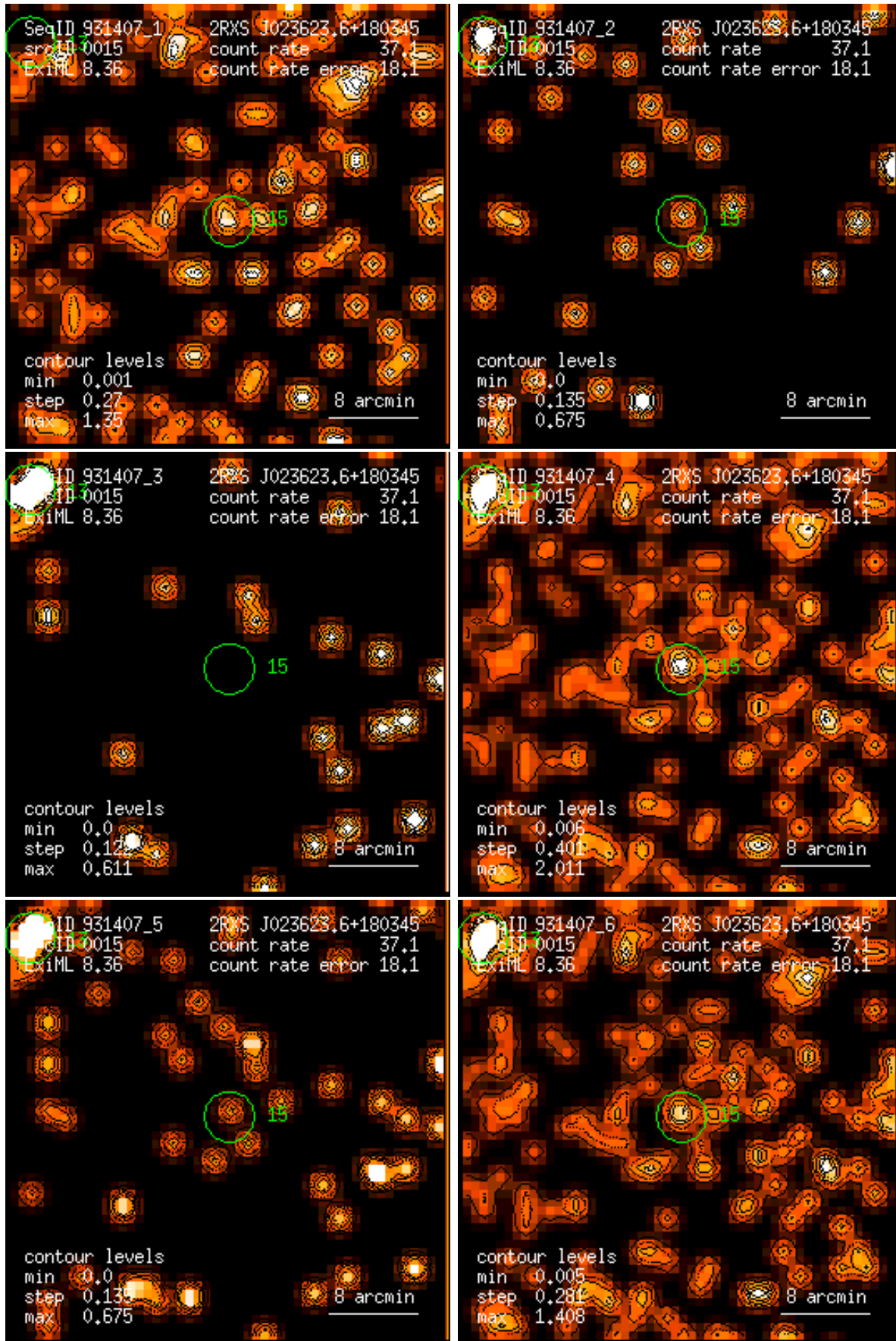
Figure 15: RASS 931407: detection 0015: band rate images, Gaussian filter: (1) PSPC channels 11 – 41, (2) 52 – 90, (3) 91 – 201, (4) 11 – 235, (5) 52 – 201, (6) 11 – 201. Broad band rates in counts/ks. Band rate contour levels in counts/ks/arcmin 2 .
