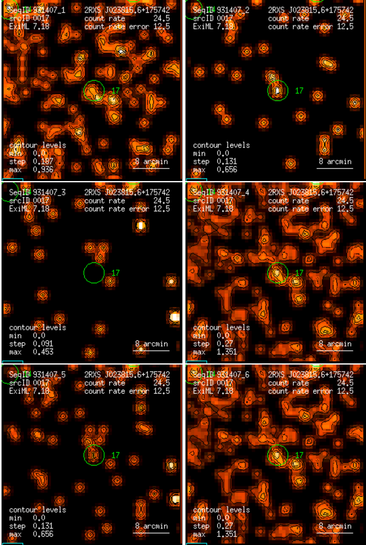
Figure 17: RASS 931407: detection 0017: band rate images, Gaussian filter: (1) PSPC channels 11 – 41, (2) 52 – 90, (3) 91 – 201, (4) 11 – 235, (5) 52 – 201, (6) 11 – 201. Broad band rates in counts/ks. Band rate contour levels in counts/ks/arcmin 2 .
