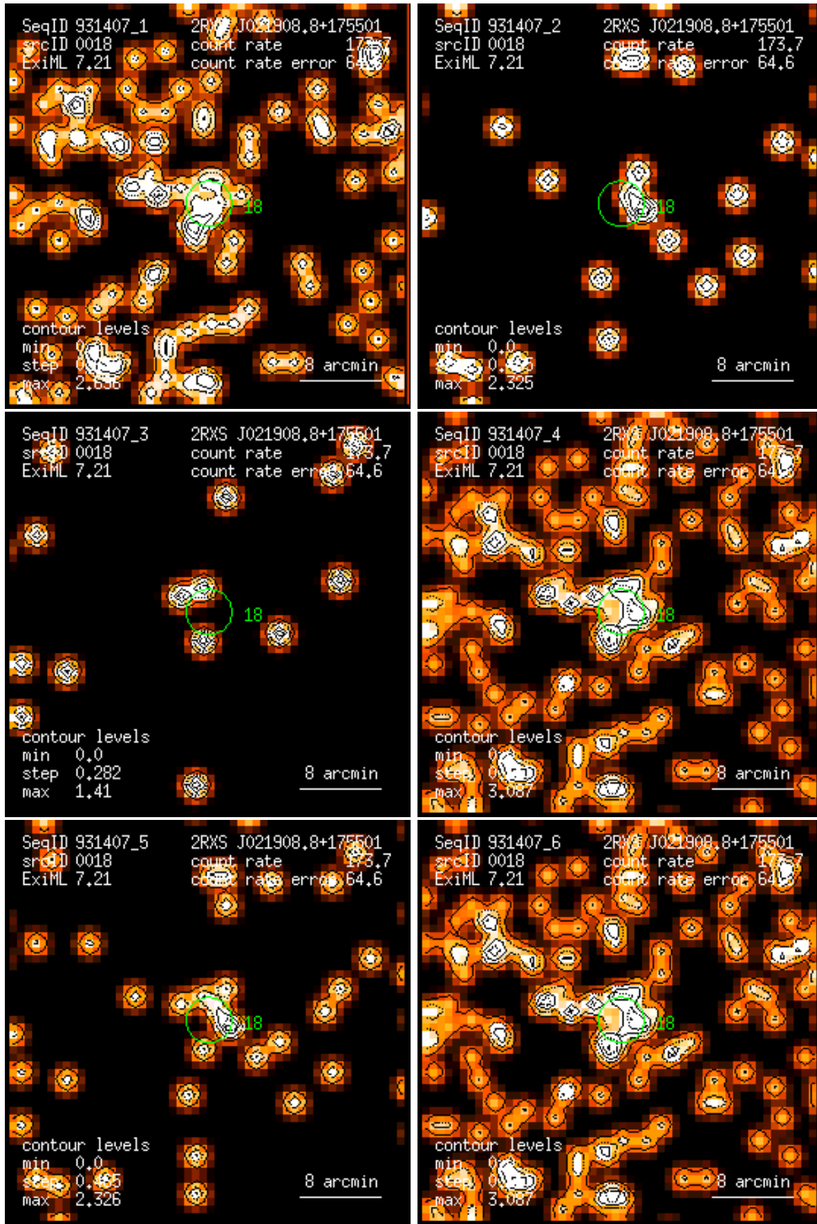
Figure 18: RASS 931407: detection 0018: band rate images, Gaussian filter: (1) PSPC channels 11 – 41, (2) 52 – 90, (3) 91 – 201, (4) 11 – 235, (5) 52 – 201, (6) 11 – 201. Broad band rates in counts/ks. Band rate contour levels in counts/ks/arcmin 2 .
