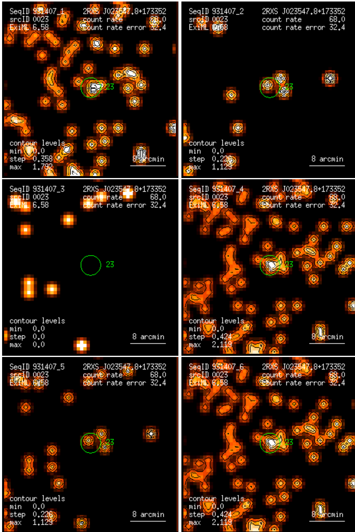
Figure 23: RASS 931407: detection 0023: band rate images, Gaussian filter: (1) PSPC channels 11 – 41, (2) 52 – 90, (3) 91 – 201, (4) 11 – 235, (5) 52 – 201, (6) 11 – 201. Broad band rates in counts/ks. Band rate contour levels in counts/ks/arcmin 2 .
