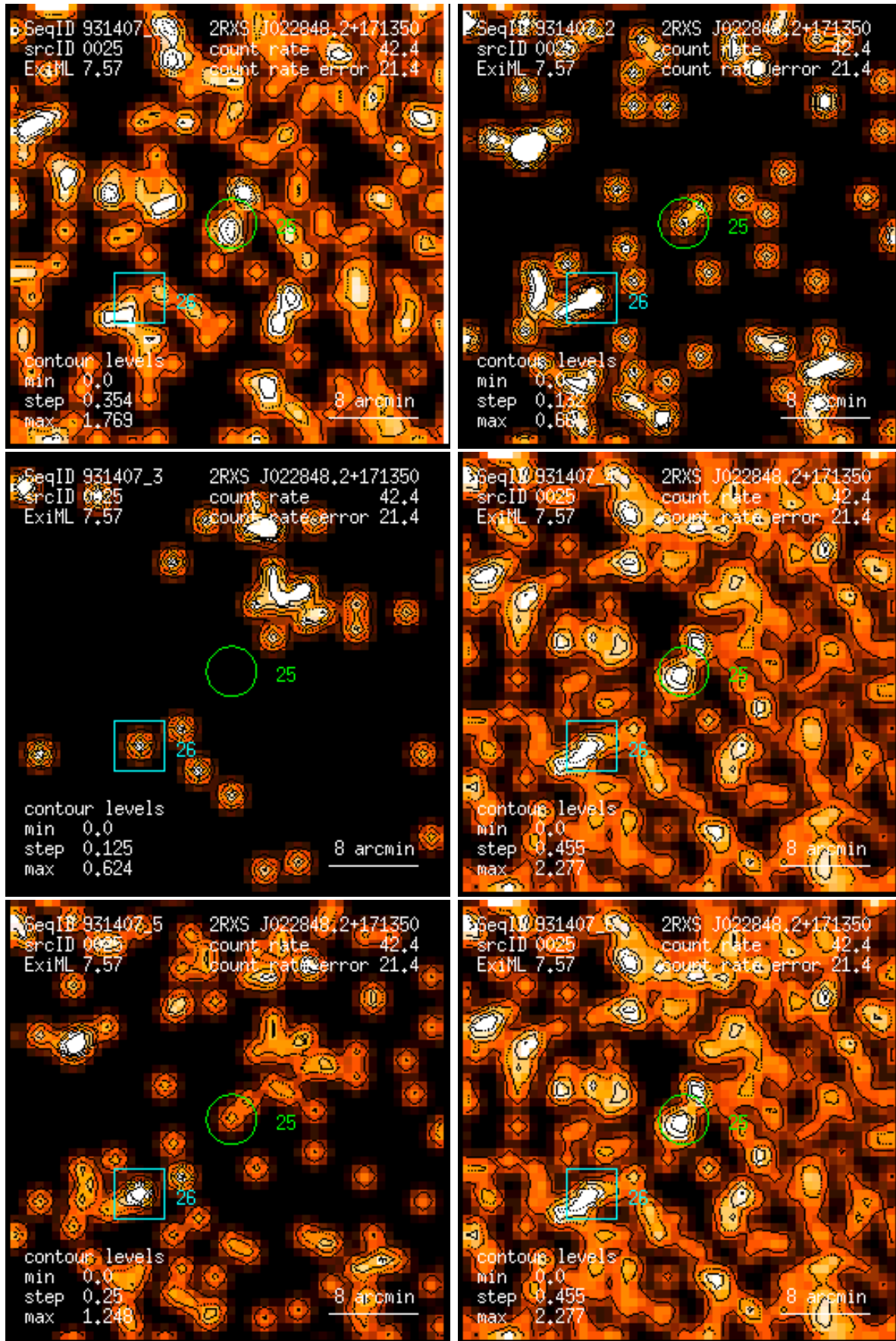
Figure 25: RASS 931407: detection 0025: band rate images, Gaussian filter: (1) PSPC channels 11 – 41, (2) 52 – 90, (3) 91 – 201, (4) 11 – 235, (5) 52 – 201, (6) 11 – 201. Broad band rates in counts/ks. Band rate contour levels in counts/ks/arcmin 2 .
