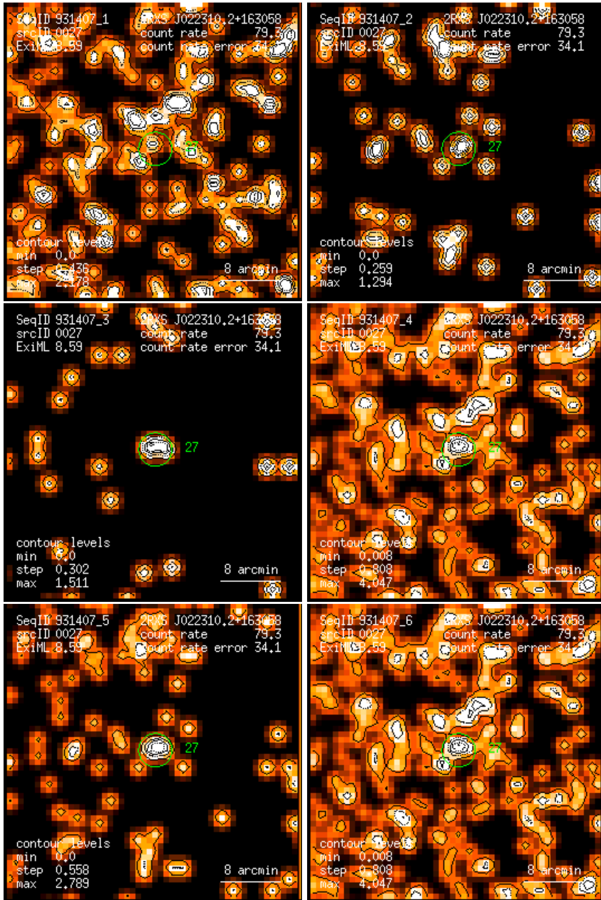
Figure 27: RASS 931407: detection 0027: band rate images, Gaussian filter: (1) PSPC channels 11 – 41, (2) 52 – 90, (3) 91 – 201, (4) 11 – 235, (5) 52 – 201, (6) 11 – 201. Broad band rates in counts/ks. Band rate contour levels in counts/ks/arcmin 2 .
