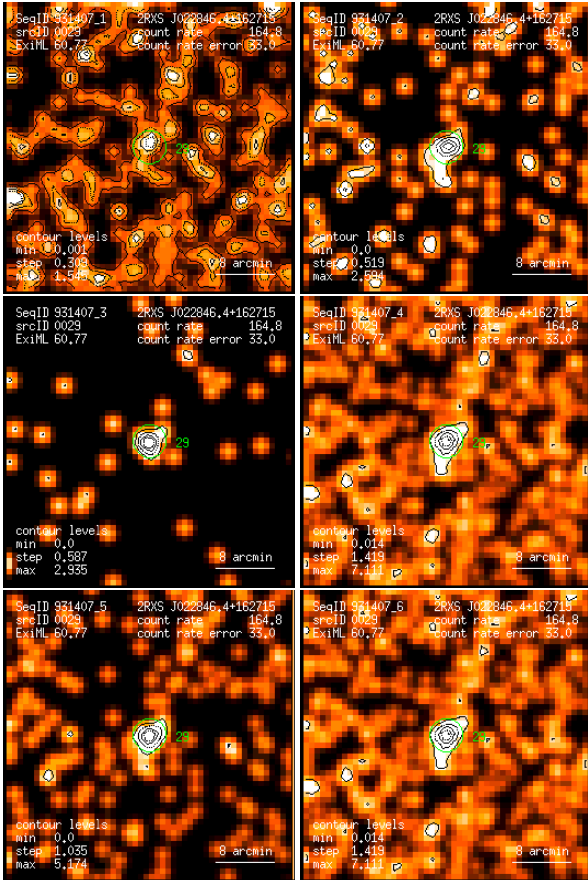
Figure 29: RASS 931407: detection 0029: band rate images, Gaussian filter: (1) PSPC channels 11 – 41, (2) 52 – 90, (3) 91 – 201, (4) 11 – 235, (5) 52 – 201, (6) 11 – 201. Broad band rates in counts/ks. Band rate contour levels in counts/ks/arcmin 2 .
