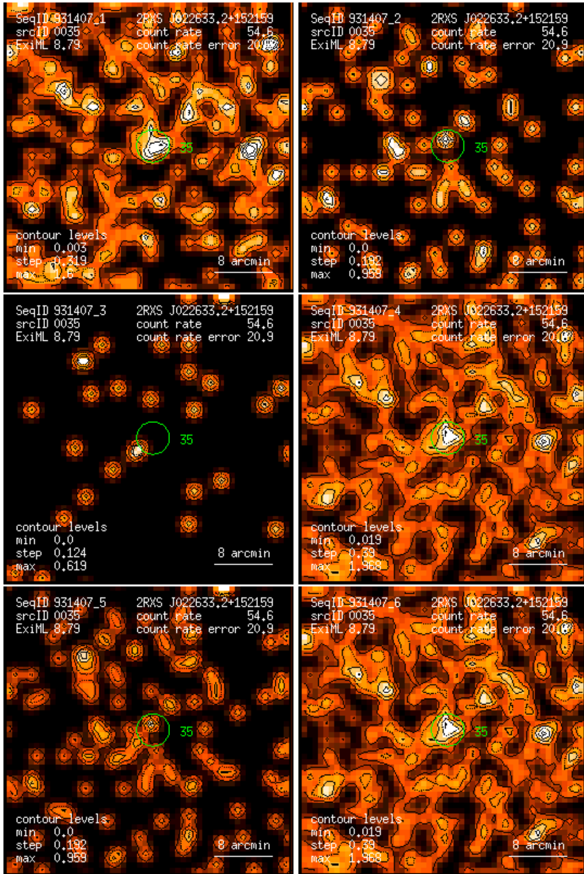
Figure 35: RASS 931407: detection 0035: band rate images, Gaussian filter: (1) PSPC channels 11 – 41, (2) 52 – 90, (3) 91 – 201, (4) 11 – 235, (5) 52 – 201, (6) 11 – 201. Broad band rates in counts/ks. Band rate contour levels in counts/ks/arcmin 2 .
