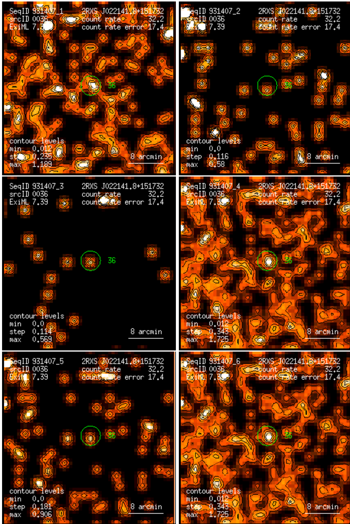
Figure 36: RASS 931407: detection 0036: band rate images, Gaussian filter: (1) PSPC channels 11 – 41, (2) 52 – 90, (3) 91 – 201, (4) 11 – 235, (5) 52 – 201, (6) 11 – 201. Broad band rates in counts/ks. Band rate contour levels in counts/ks/arcmin 2 .
