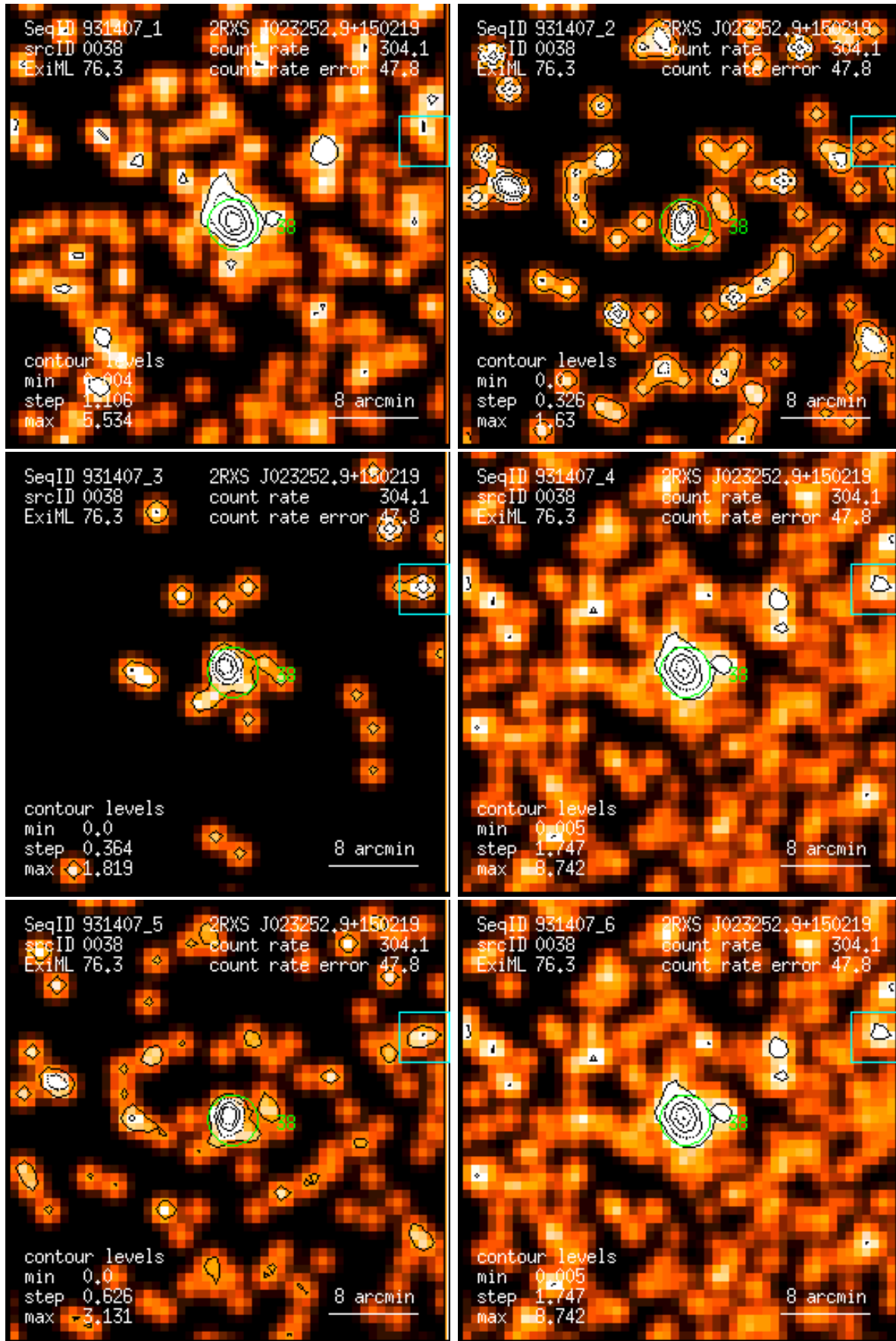
Figure 38: RASS 931407: detection 0038: band rate images, Gaussian filter: (1) PSPC channels 11 – 41, (2) 52 – 90, (3) 91 – 201, (4) 11 – 235, (5) 52 – 201, (6) 11 – 201. Broad band rates in counts/ks. Band rate contour levels in counts/ks/arcmin 2 .
