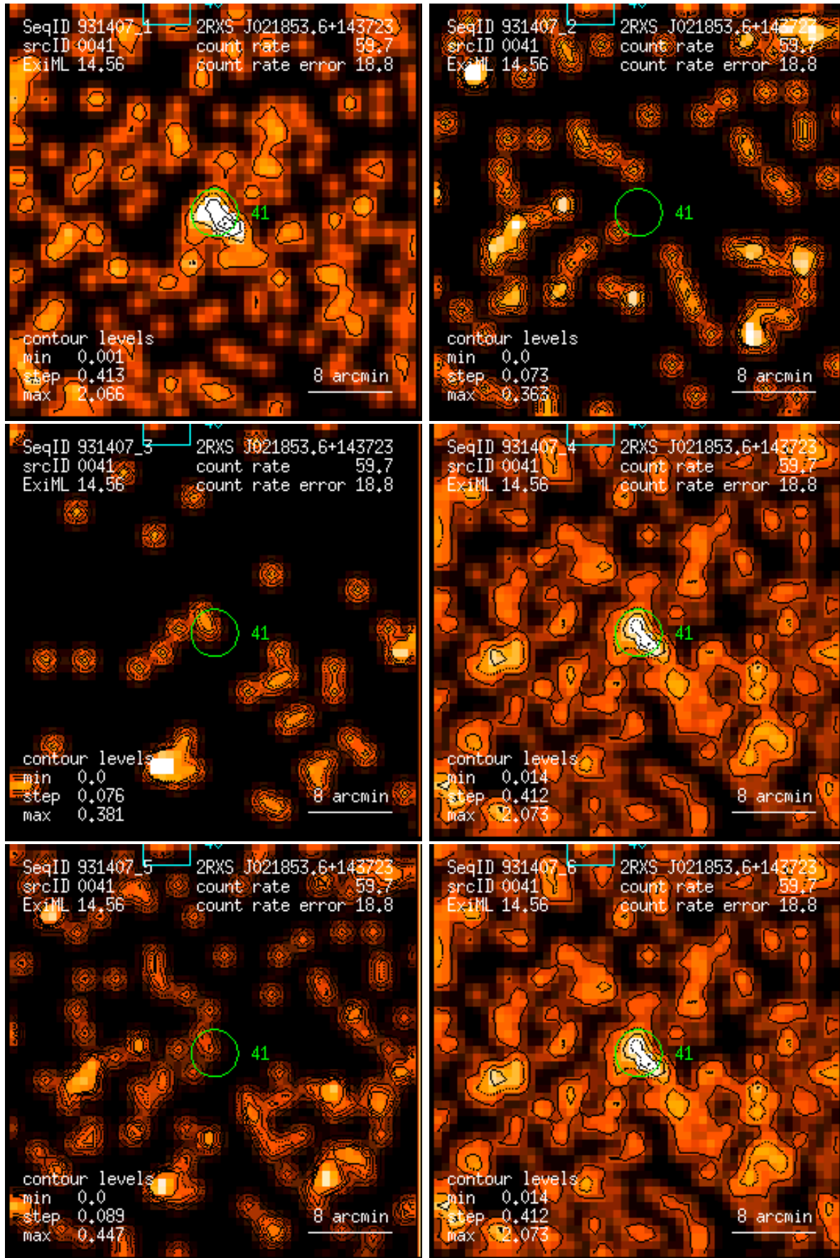
Figure 41: RASS 931407: detection 0041: band rate images, Gaussian filter: (1) PSPC channels 11 – 41, (2) 52 – 90, (3) 91 – 201, (4) 11 – 235, (5) 52 – 201, (6) 11 – 201. Broad band rates in counts/ks. Band rate contour levels in counts/ks/arcmin 2 .
