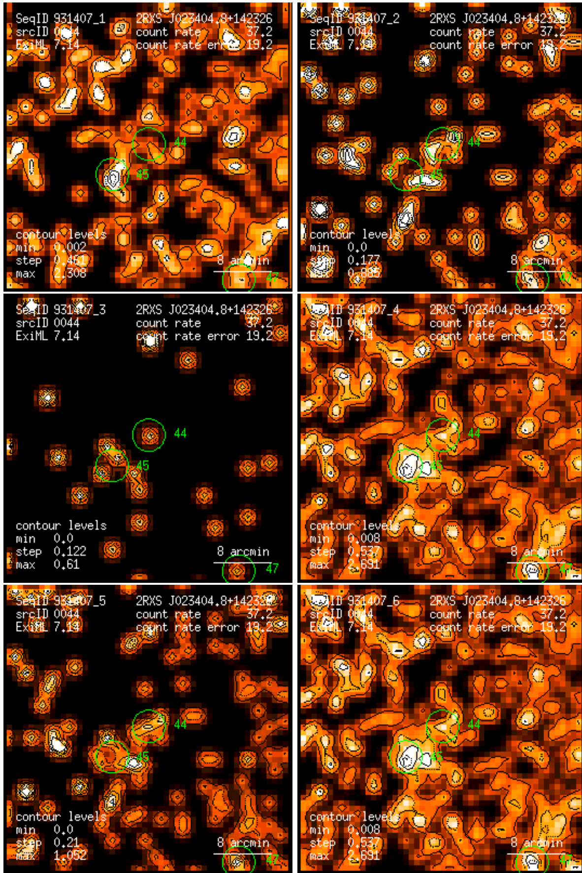
Figure 44: RASS 931407: detection 0044: band rate images, Gaussian filter: (1) PSPC channels 11 – 41, (2) 52 – 90, (3) 91 – 201, (4) 11 – 235, (5) 52 – 201, (6) 11 – 201. Broad band rates in counts/ks. Band rate contour levels in counts/ks/arcmin 2 .
