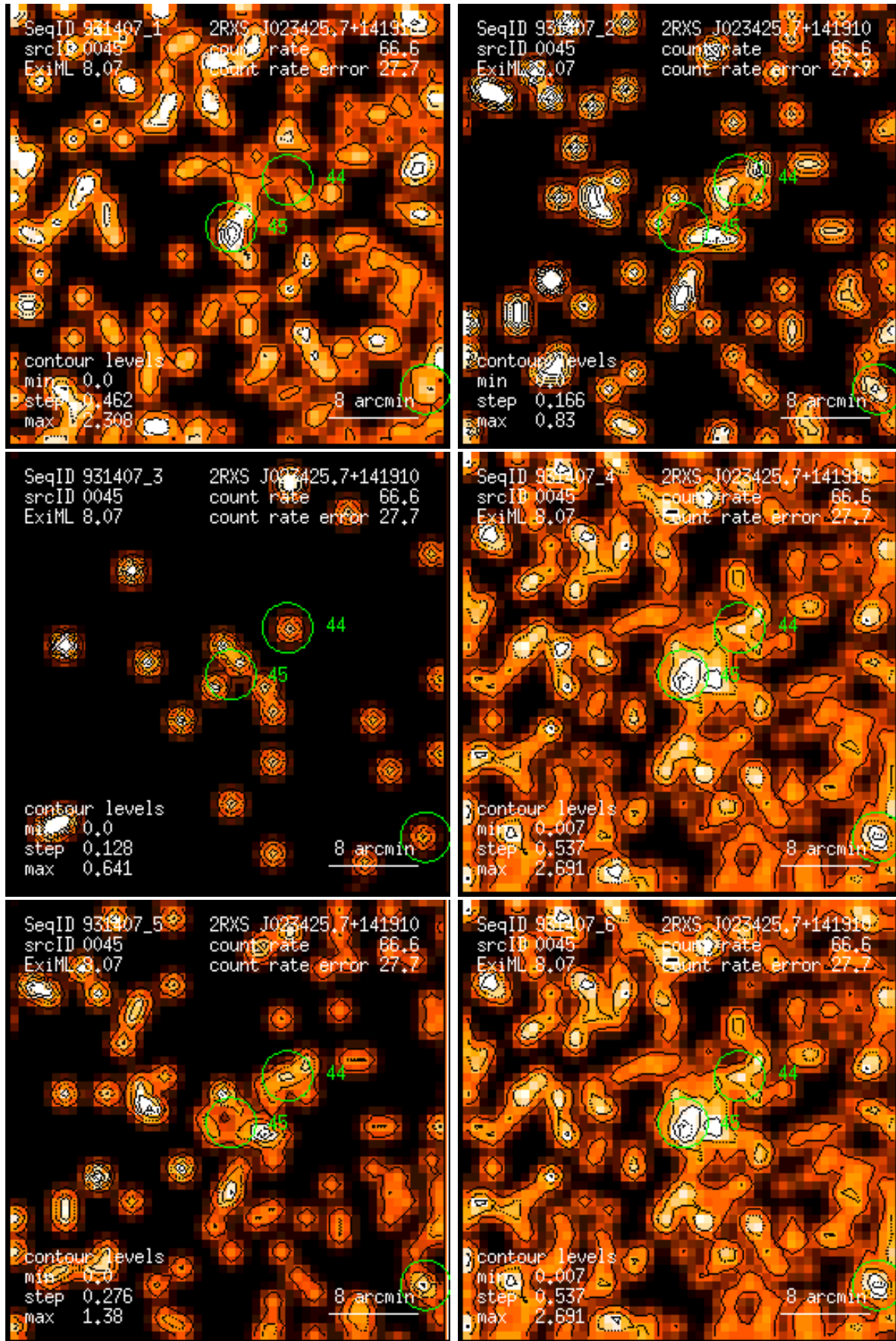
Figure 45: RASS 931407: detection 0045: band rate images, Gaussian filter: (1) PSPC channels 11 – 41, (2) 52 – 90, (3) 91 – 201, (4) 11 – 235, (5) 52 – 201, (6) 11 – 201. Broad band rates in counts/ks. Band rate contour levels in counts/ks/arcmin 2 .
