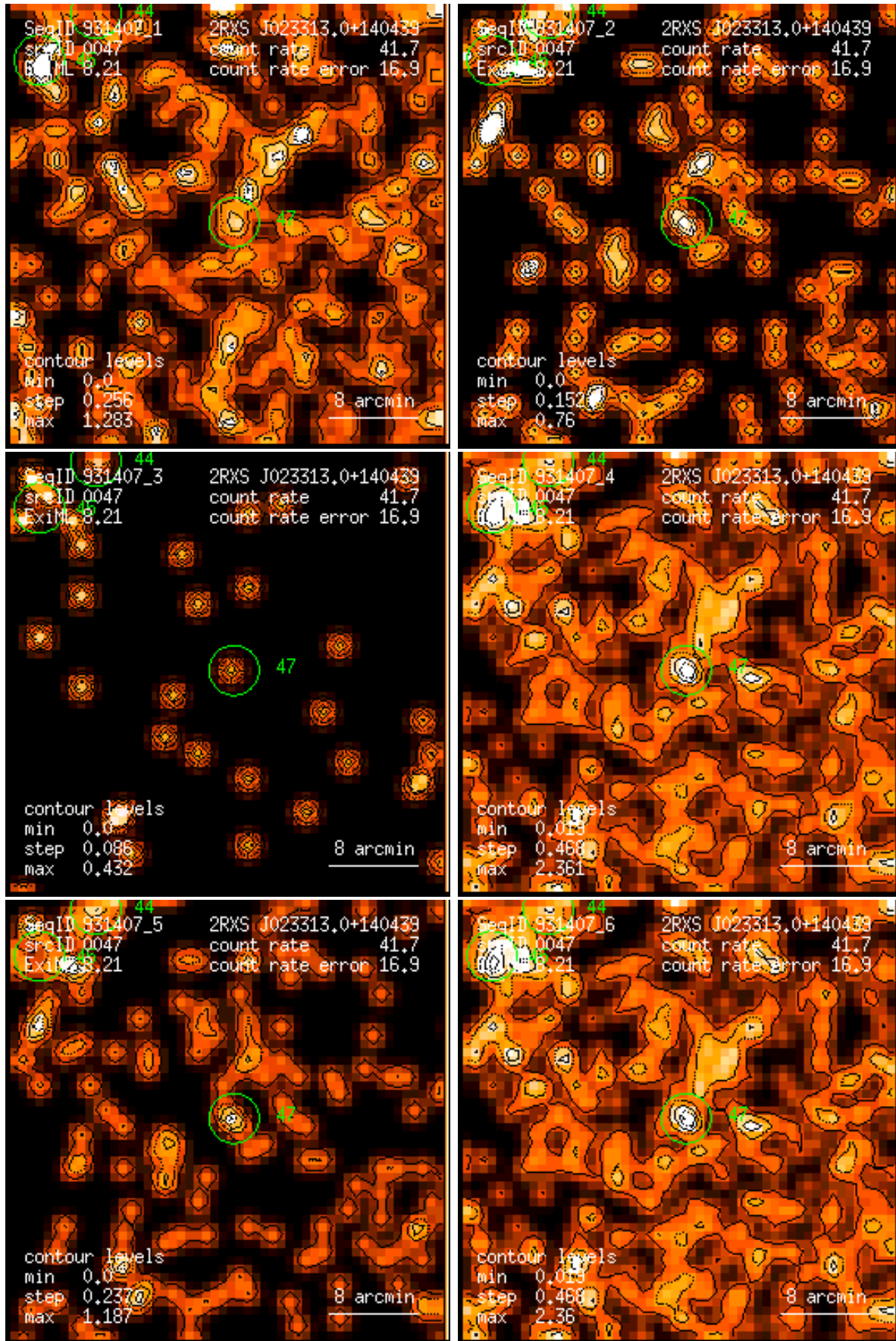
Figure 47: RASS 931407: detection 0047: band rate images, Gaussian filter: (1) PSPC channels 11 – 41, (2) 52 – 90, (3) 91 – 201, (4) 11 – 235, (5) 52 – 201, (6) 11 – 201. Broad band rates in counts/ks. Band rate contour levels in counts/ks/arcmin 2 .
