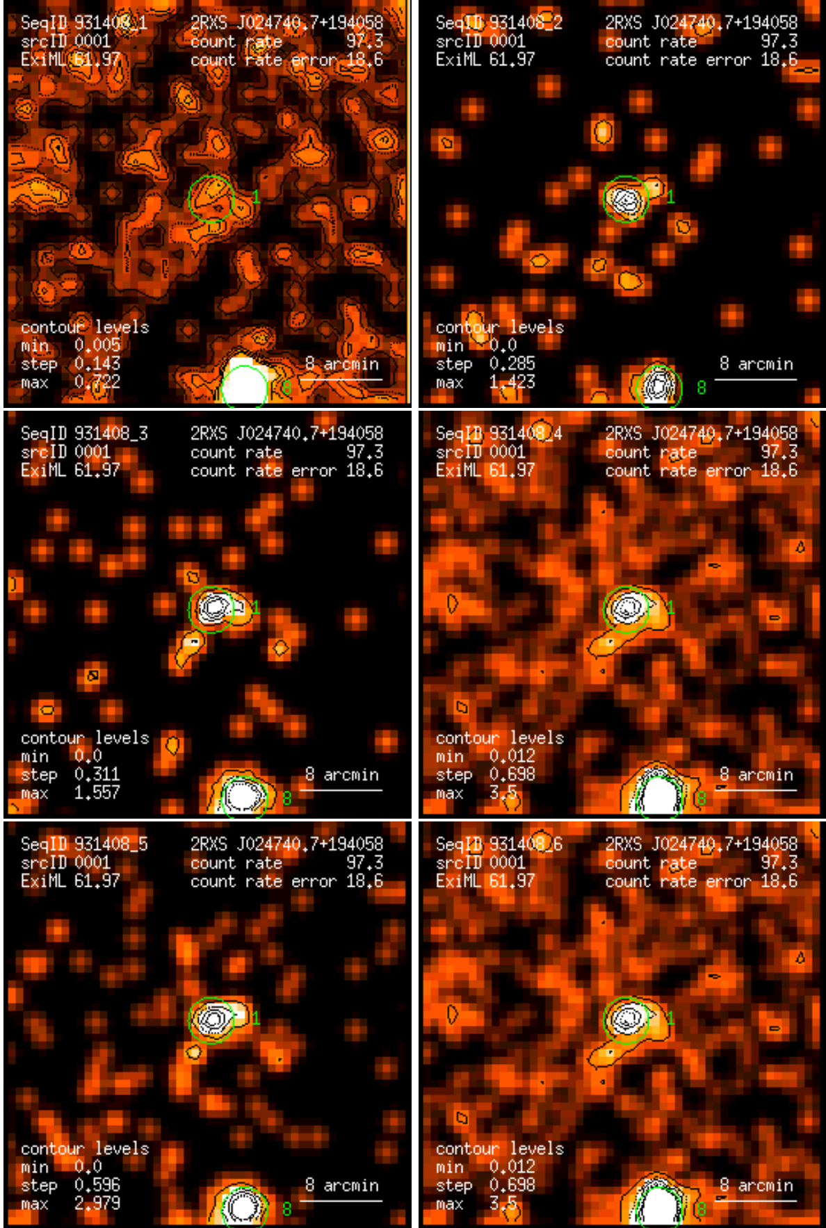
Figure 1: RASS 931408: detection 0001: band rate images, Gaussian filter: (1) PSPC channels 11 – 41, (2) 52 – 90, (3) 91 – 201, (4) 11 – 235, (5) 52 – 201, (6) 11 – 201. Broad band rates in counts/ks. Band rate contour levels in counts/ks/arcmin 2 .
