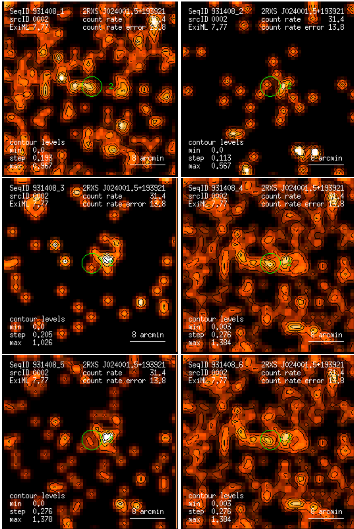
Figure 2: RASS 931408: detection 0002: band rate images, Gaussian filter: (1) PSPC channels 11 – 41, (2) 52 – 90, (3) 91 – 201, (4) 11 – 235, (5) 52 – 201, (6) 11 – 201. Broad band rates in counts/ks. Band rate contour levels in counts/ks/arcmin 2 .
