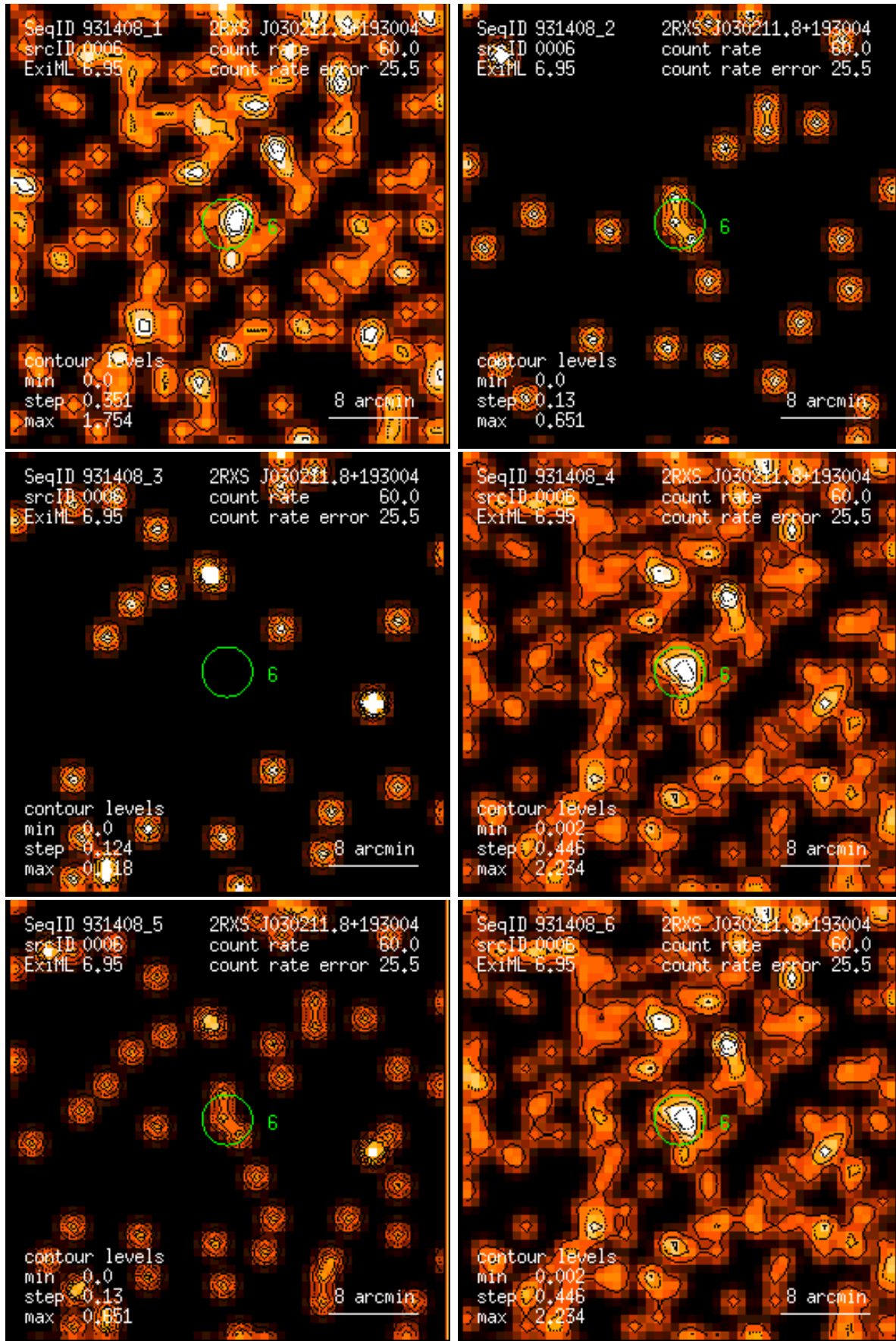
Figure 6: RASS 931408: detection 0006: band rate images, Gaussian filter: (1) PSPC channels 11 – 41, (2) 52 – 90, (3) 91 – 201, (4) 11 – 235, (5) 52 – 201, (6) 11 – 201. Broad band rates in counts/ks. Band rate contour levels in counts/ks/arcmin 2 .
