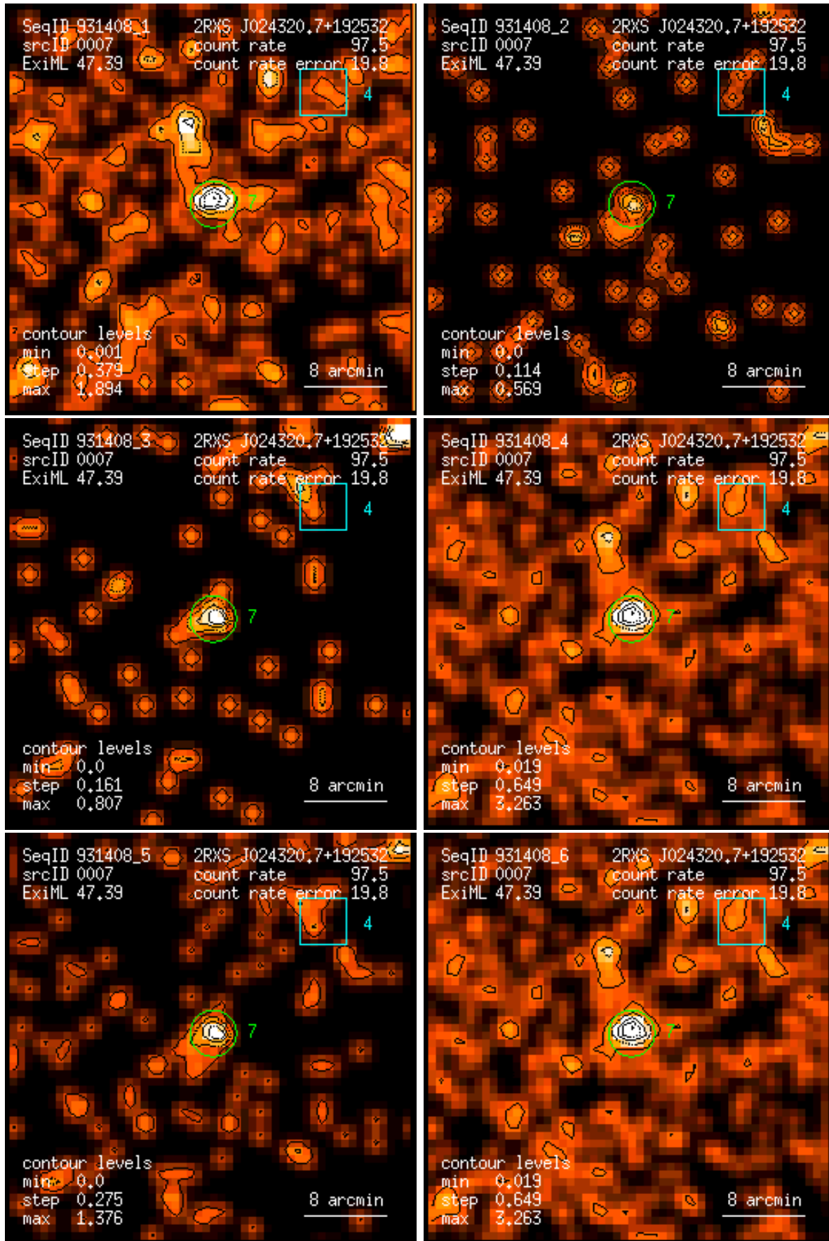
Figure 7: RASS 931408: detection 0007: band rate images, Gaussian filter: (1) PSPC channels 11 – 41, (2) 52 – 90, (3) 91 – 201, (4) 11 – 235, (5) 52 – 201, (6) 11 – 201. Broad band rates in counts/ks. Band rate contour levels in counts/ks/arcmin 2 .
