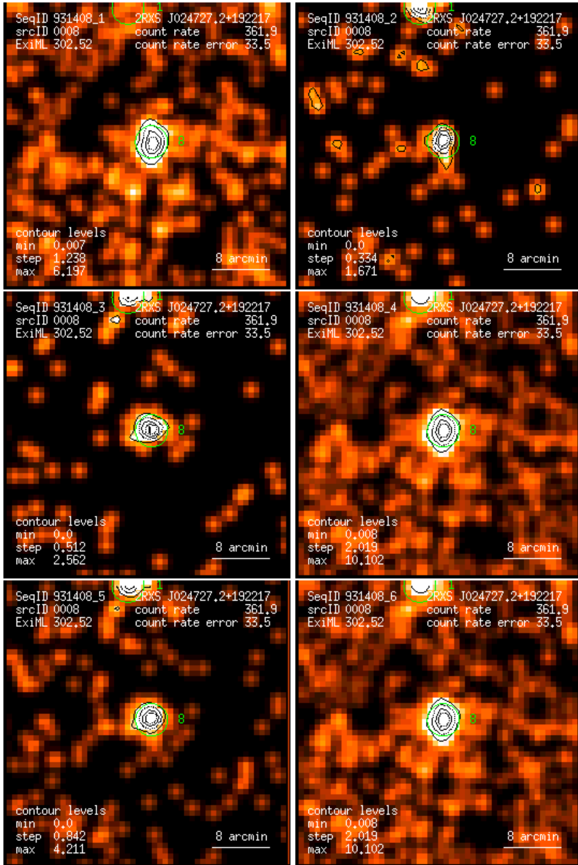
Figure 8: RASS 931408: detection 0008: band rate images, Gaussian filter: (1) PSPC channels 11 – 41, (2) 52 – 90, (3) 91 – 201, (4) 11 – 235, (5) 52 – 201, (6) 11 – 201. Broad band rates in counts/ks. Band rate contour levels in counts/ks/arcmin 2 .
