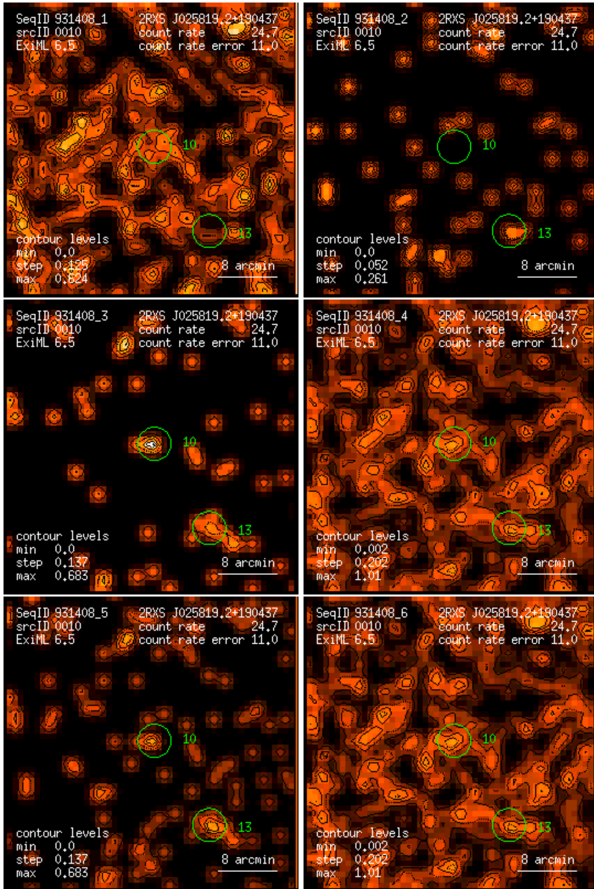
Figure 10: RASS 931408: detection 0010: band rate images, Gaussian filter: (1) PSPC channels 11 – 41, (2) 52 – 90, (3) 91 – 201, (4) 11 – 235, (5) 52 – 201, (6) 11 – 201. Broad band rates in counts/ks. Band rate contour levels in counts/ks/arcmin 2 .
