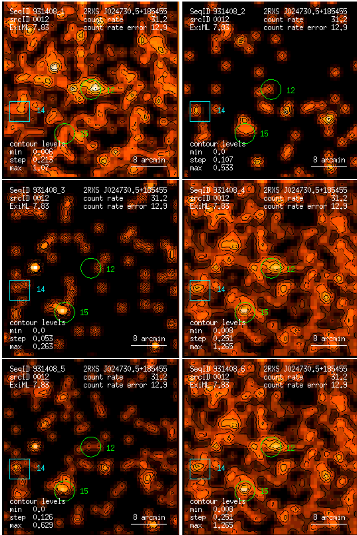
Figure 12: RASS 931408: detection 0012: band rate images, Gaussian filter: (1) PSPC channels 11 – 41, (2) 52 – 90, (3) 91 – 201, (4) 11 – 235, (5) 52 – 201, (6) 11 – 201. Broad band rates in counts/ks. Band rate contour levels in counts/ks/arcmin 2 .
