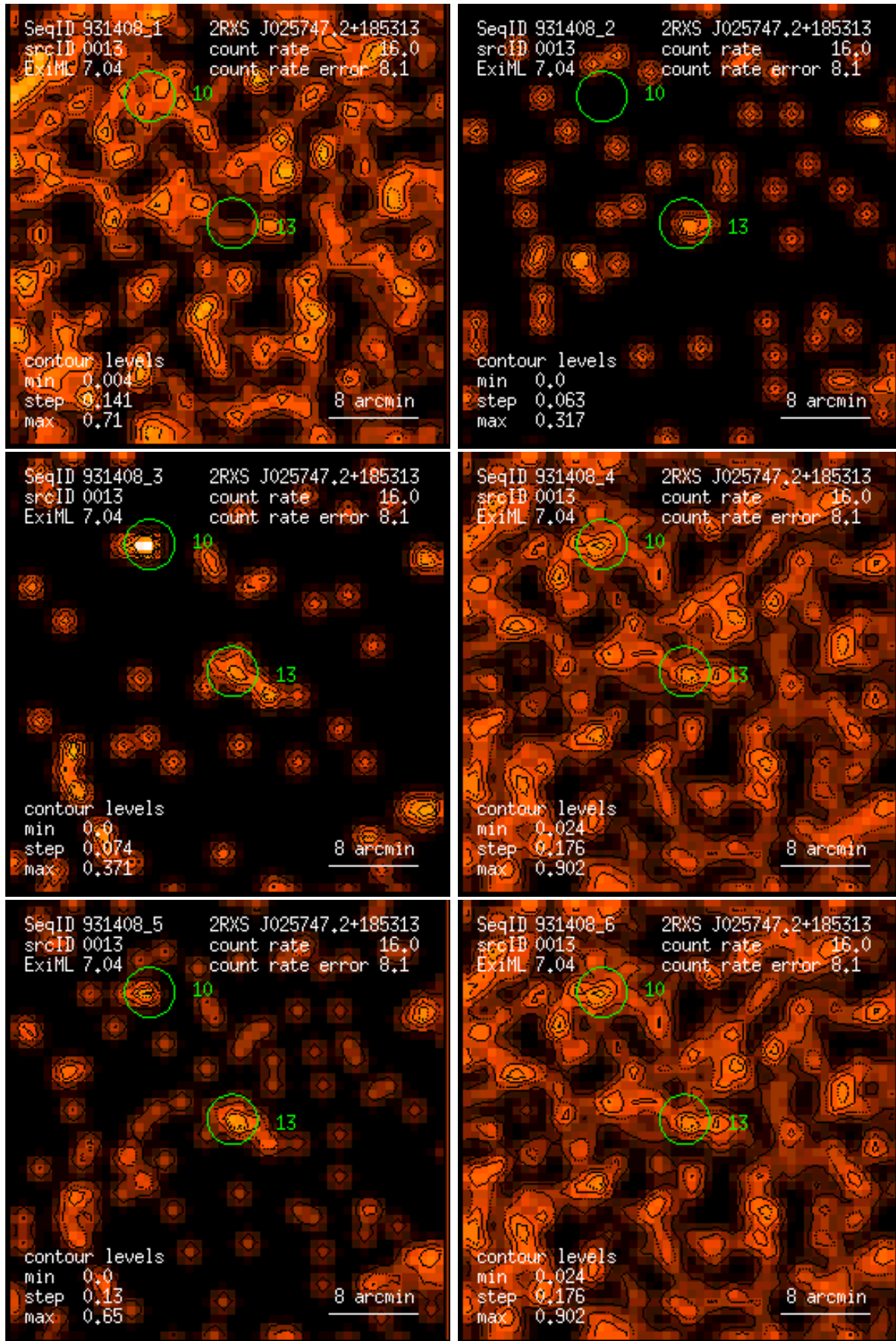
Figure 13: RASS 931408: detection 0013: band rate images, Gaussian filter: (1) PSPC channels 11 – 41, (2) 52 – 90, (3) 91 – 201, (4) 11 – 235, (5) 52 – 201, (6) 11 – 201. Broad band rates in counts/ks. Band rate contour levels in counts/ks/arcmin 2 .
