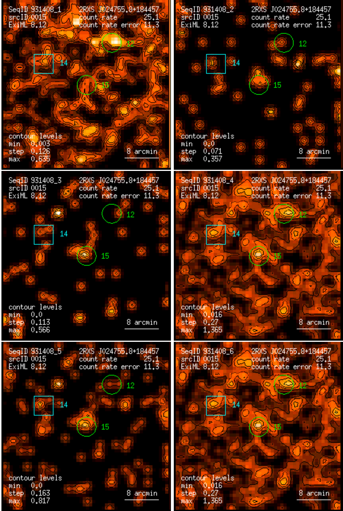
Figure 15: RASS 931408: detection 0015: band rate images, Gaussian filter: (1) PSPC channels 11 – 41, (2) 52 – 90, (3) 91 – 201, (4) 11 – 235, (5) 52 – 201, (6) 11 – 201. Broad band rates in counts/ks. Band rate contour levels in counts/ks/arcmin 2 .
