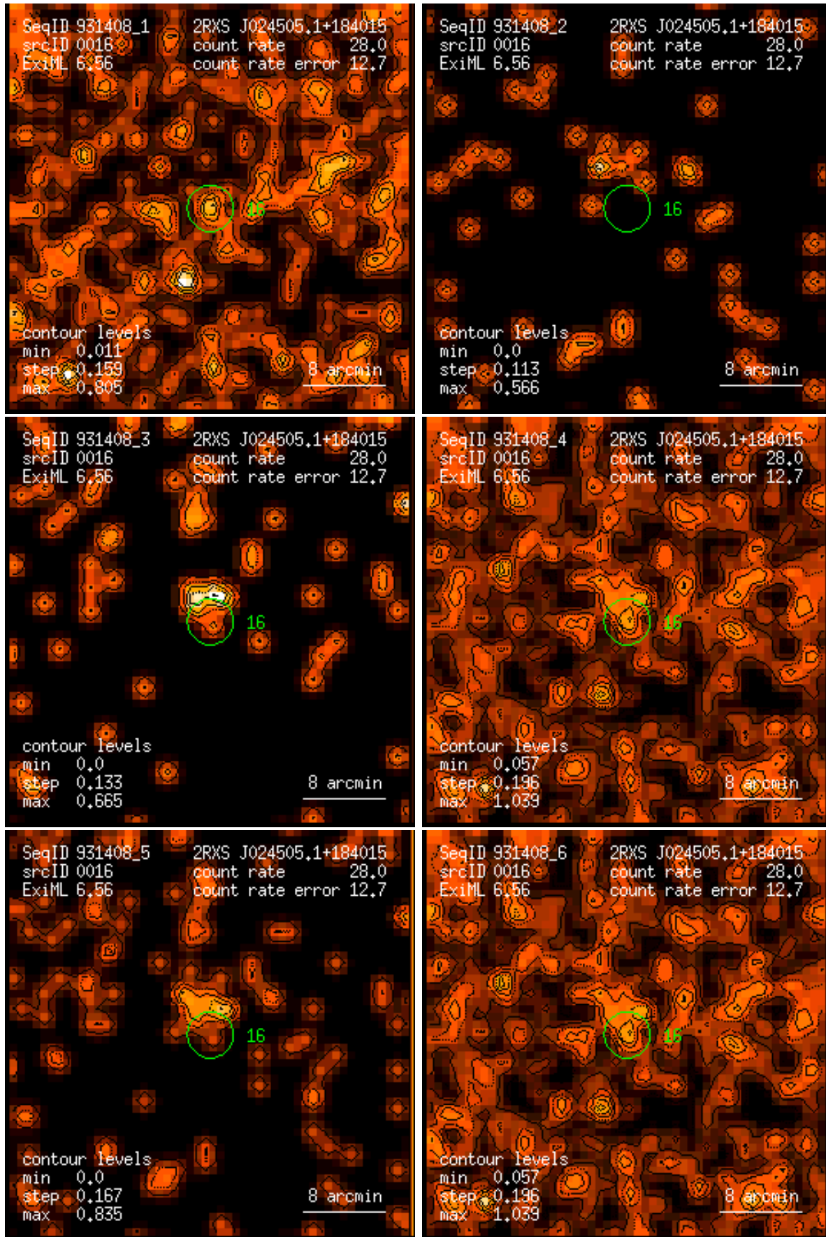
Figure 16: RASS 931408: detection 0016: band rate images, Gaussian filter: (1) PSPC channels 11 – 41, (2) 52 – 90, (3) 91 – 201, (4) 11 – 235, (5) 52 – 201, (6) 11 – 201. Broad band rates in counts/ks. Band rate contour levels in counts/ks/arcmin 2 .
