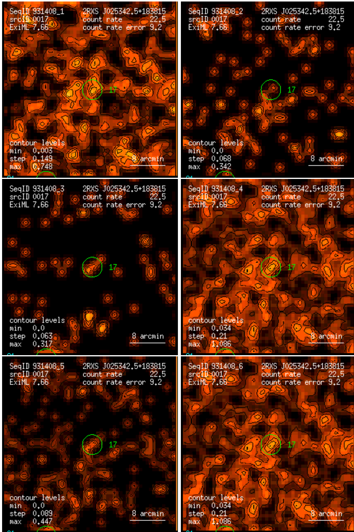
Figure 17: RASS 931408: detection 0017: band rate images, Gaussian filter: (1) PSPC channels 11 – 41, (2) 52 – 90, (3) 91 – 201, (4) 11 – 235, (5) 52 – 201, (6) 11 – 201. Broad band rates in counts/ks. Band rate contour levels in counts/ks/arcmin 2 .
