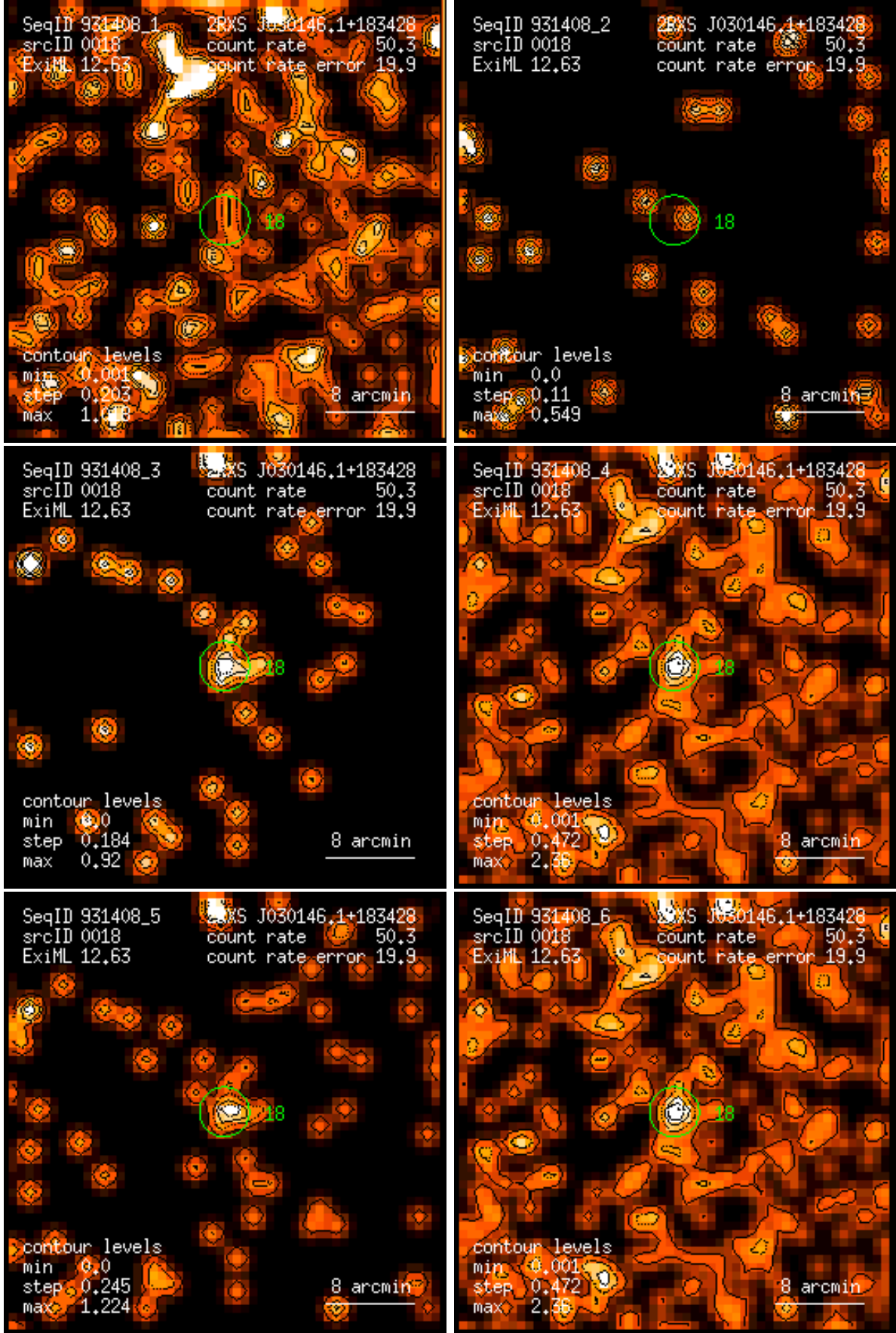
Figure 18: RASS 931408: detection 0018: band rate images, Gaussian filter: (1) PSPC channels 11 – 41, (2) 52 – 90, (3) 91 – 201, (4) 11 – 235, (5) 52 – 201, (6) 11 – 201. Broad band rates in counts/ks. Band rate contour levels in counts/ks/arcmin 2 .
