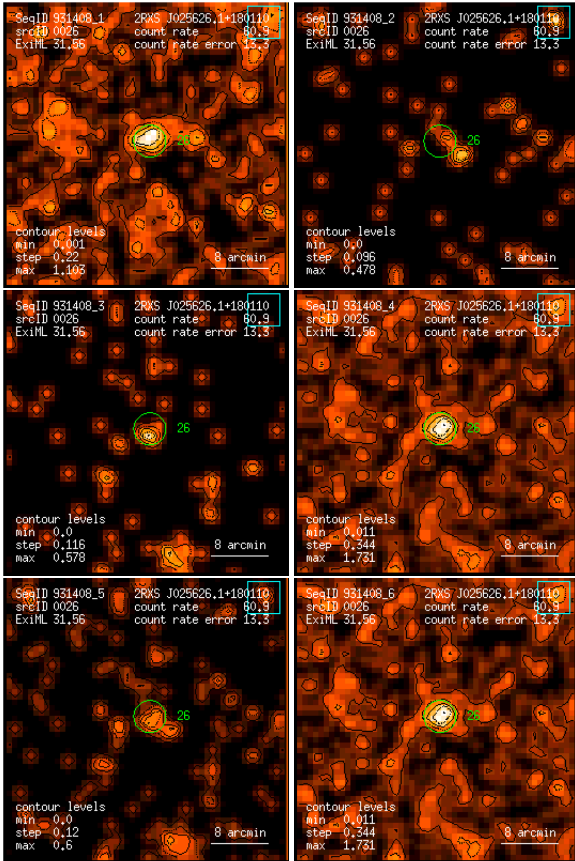
Figure 26: RASS 931408: detection 0026: band rate images, Gaussian filter: (1) PSPC channels 11 – 41, (2) 52 – 90, (3) 91 – 201, (4) 11 – 235, (5) 52 – 201, (6) 11 – 201. Broad band rates in counts/ks. Band rate contour levels in counts/ks/arcmin 2 .
