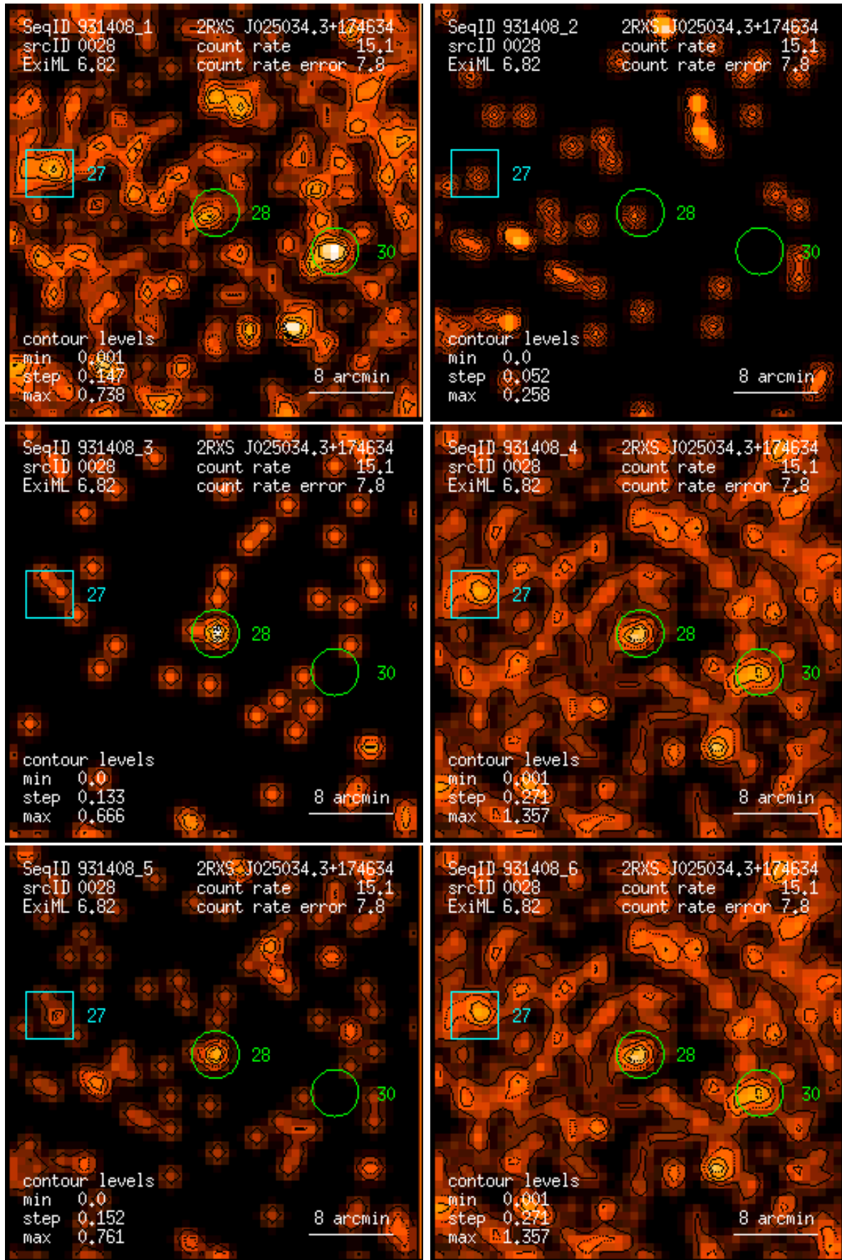
Figure 28: RASS 931408: detection 0028: band rate images, Gaussian filter: (1) PSPC channels 11 – 41, (2) 52 – 90, (3) 91 – 201, (4) 11 – 235, (5) 52 – 201, (6) 11 – 201. Broad band rates in counts/ks. Band rate contour levels in counts/ks/arcmin 2 .
