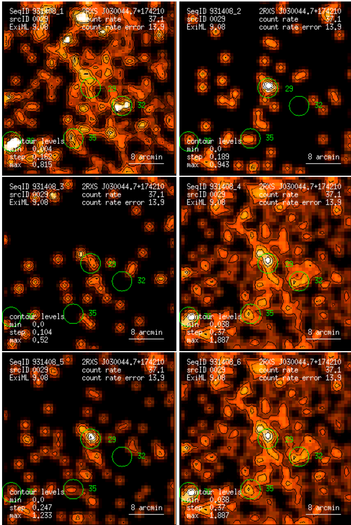
Figure 29: RASS 931408: detection 0029: band rate images, Gaussian filter: (1) PSPC channels 11 – 41, (2) 52 – 90, (3) 91 – 201, (4) 11 – 235, (5) 52 – 201, (6) 11 – 201. Broad band rates in counts/ks. Band rate contour levels in counts/ks/arcmin 2 .
