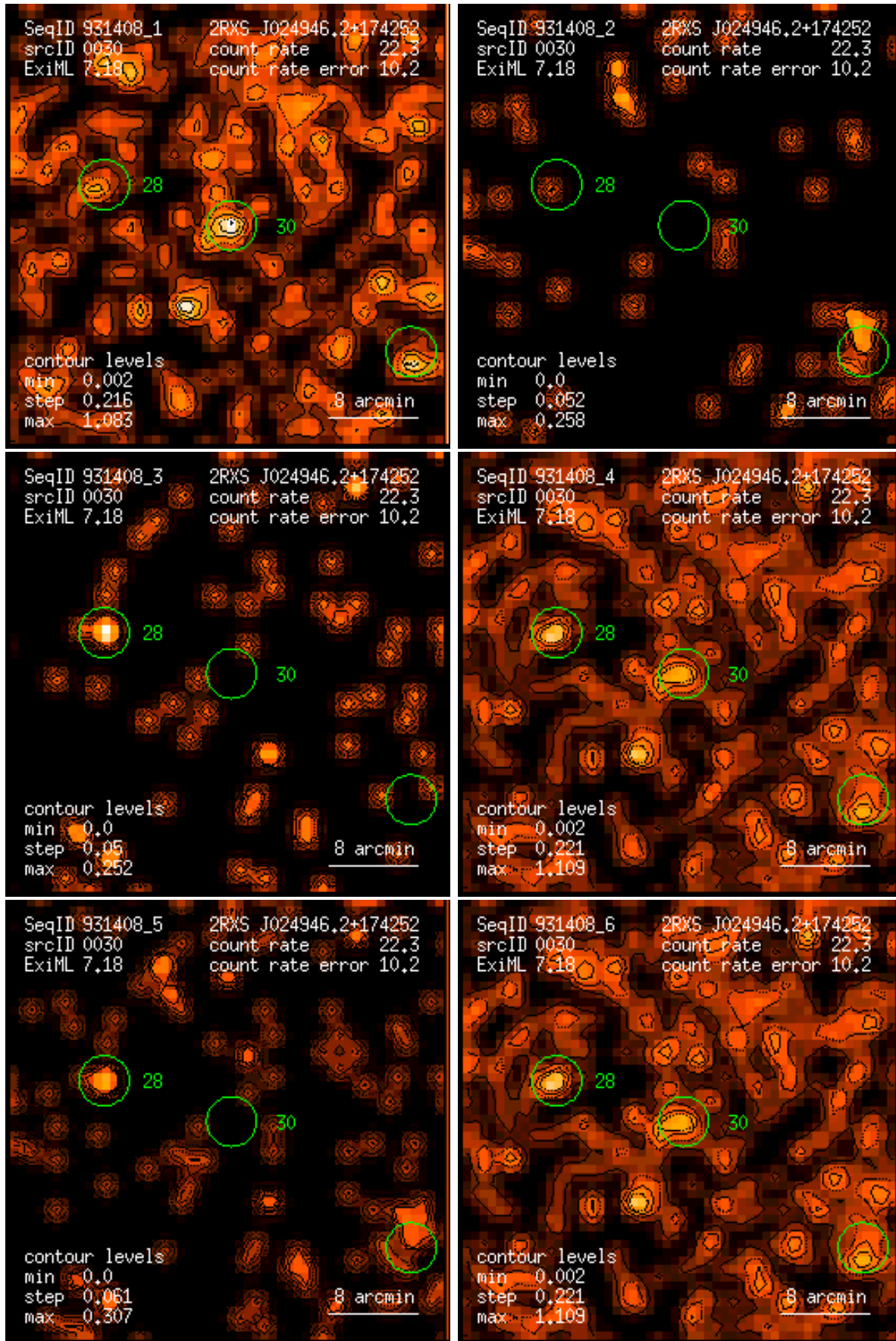
Figure 30: RASS 931408: detection 0030: band rate images, Gaussian filter: (1) PSPC channels 11 – 41, (2) 52 – 90, (3) 91 – 201, (4) 11 – 235, (5) 52 – 201, (6) 11 – 201. Broad band rates in counts/ks. Band rate contour levels in counts/ks/arcmin 2 .
