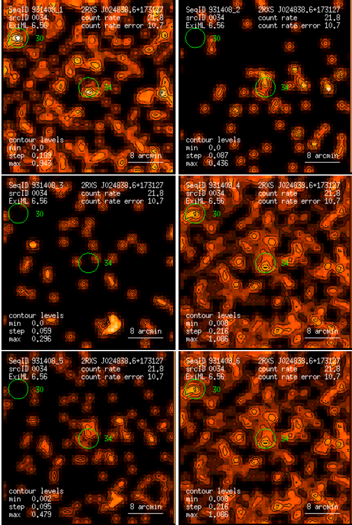
Figure 34: RASS 931408: detection 0034: band rate images, Gaussian filter: (1) PSPC channels 11 – 41, (2) 52 – 90, (3) 91 – 201, (4) 11 – 235, (5) 52 – 201, (6) 11 – 201. Broad band rates in counts/ks. Band rate contour levels in counts/ks/arcmin 2 .
