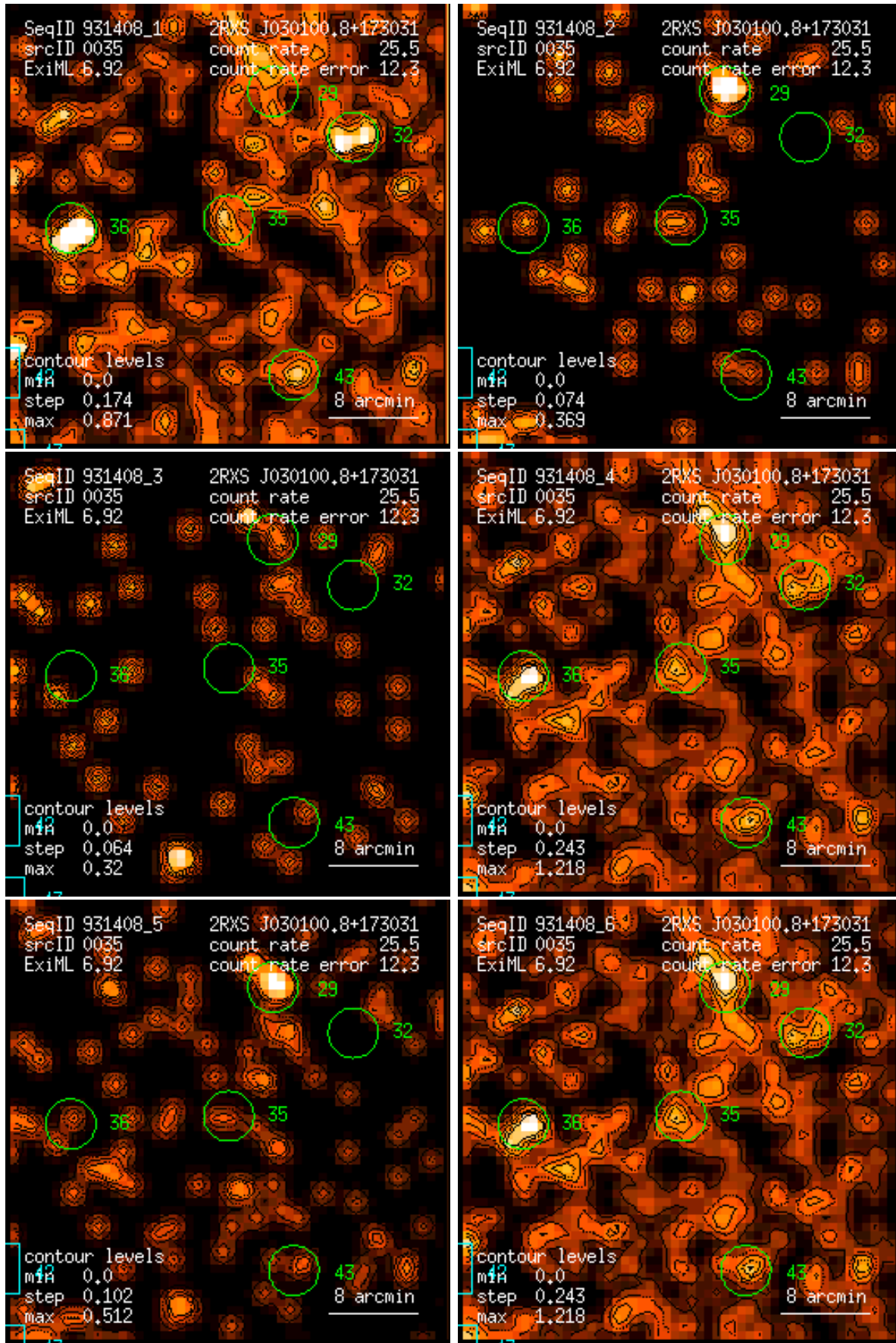
Figure 35: RASS 931408: detection 0035: band rate images, Gaussian filter: (1) PSPC channels 11 – 41, (2) 52 – 90, (3) 91 – 201, (4) 11 – 235, (5) 52 – 201, (6) 11 – 201. Broad band rates in counts/ks. Band rate contour levels in counts/ks/arcmin 2 .
